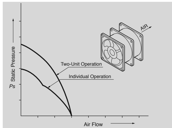
Series Operation
