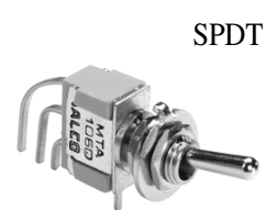
MTA8106DVRA Vertical Actuation
