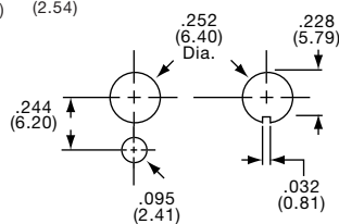
MTA8106DVRA Vertical Actuation
