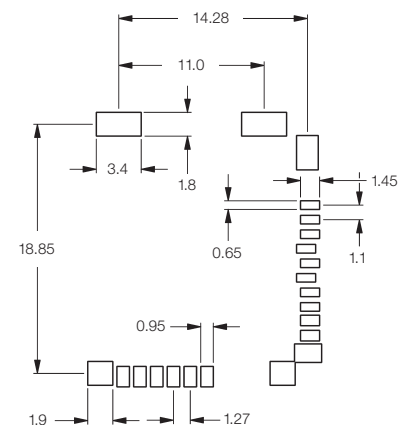
PCB Layout
