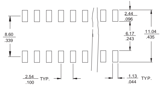
SURFACE MOUNT PAD LAYOUTS (ALL STYLES)
