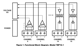
Figure 1. Functional Block Diagram, Model 7BP16-1
