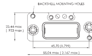
Plug With Grounding Block GPRB1WB05N
