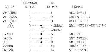
WIRING DIAGRAM
