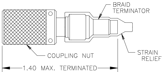
PLUG ASSEMBLY: D-621-0911
