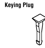
Part No. 86286-1 (Plugs into receptacle contact) Material: Natural color nylon
