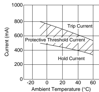
Protective Threshold Current Range
