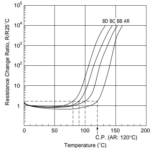
Resistance - Temperature Characteristic
