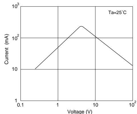
Current - Voltage Characteristic (Static Characteristic)
