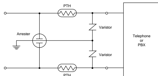
(5) Telecommunication Circuit
