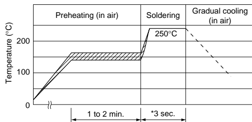
Flow Soldering Conditions
