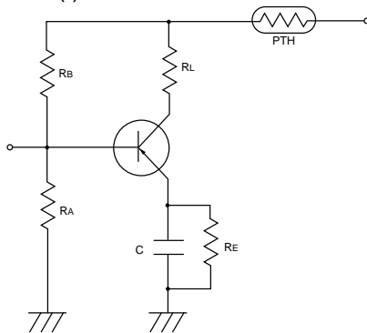
(3) Transistor Protection Circuit
