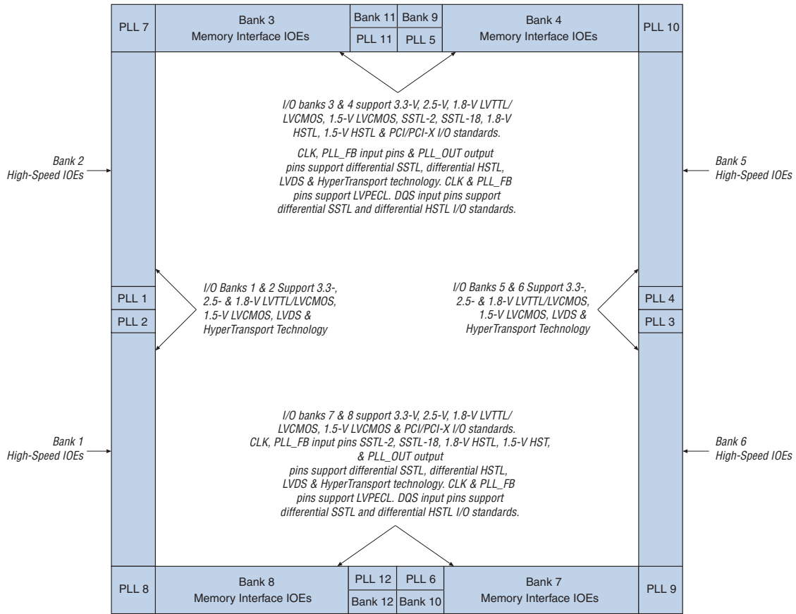
Figure 2–6. I/O Type Support in HC240 Devices Notes (1), (2)
