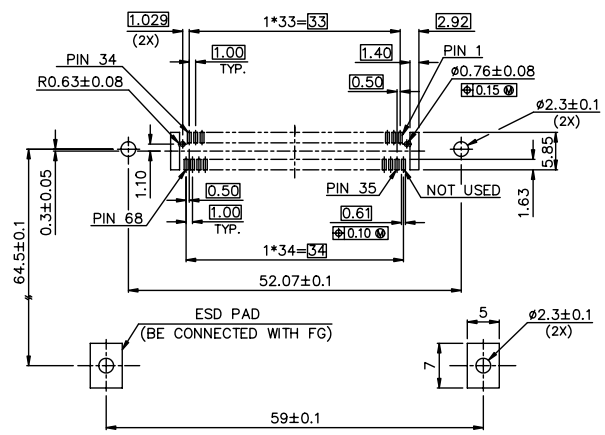
RECOMMENDED P.C.B. LAYOUT 6-2 (MOUNTED SIDE)
