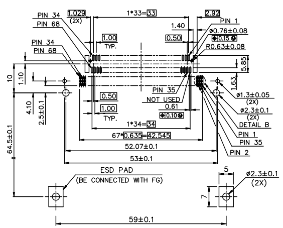
RECOMMENDED P.C.B. LAYOUT 4 (MOUNTED SIDE)
