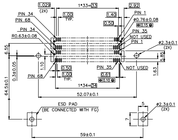
RECOMMENDED P.C.B. LAYOUT 6-1 (MOUNTED SIDE)
