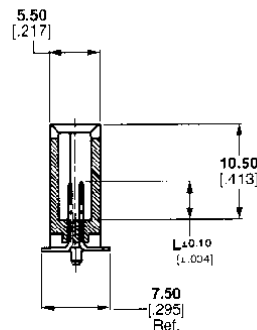
Section C - C (Rotated 90°)
