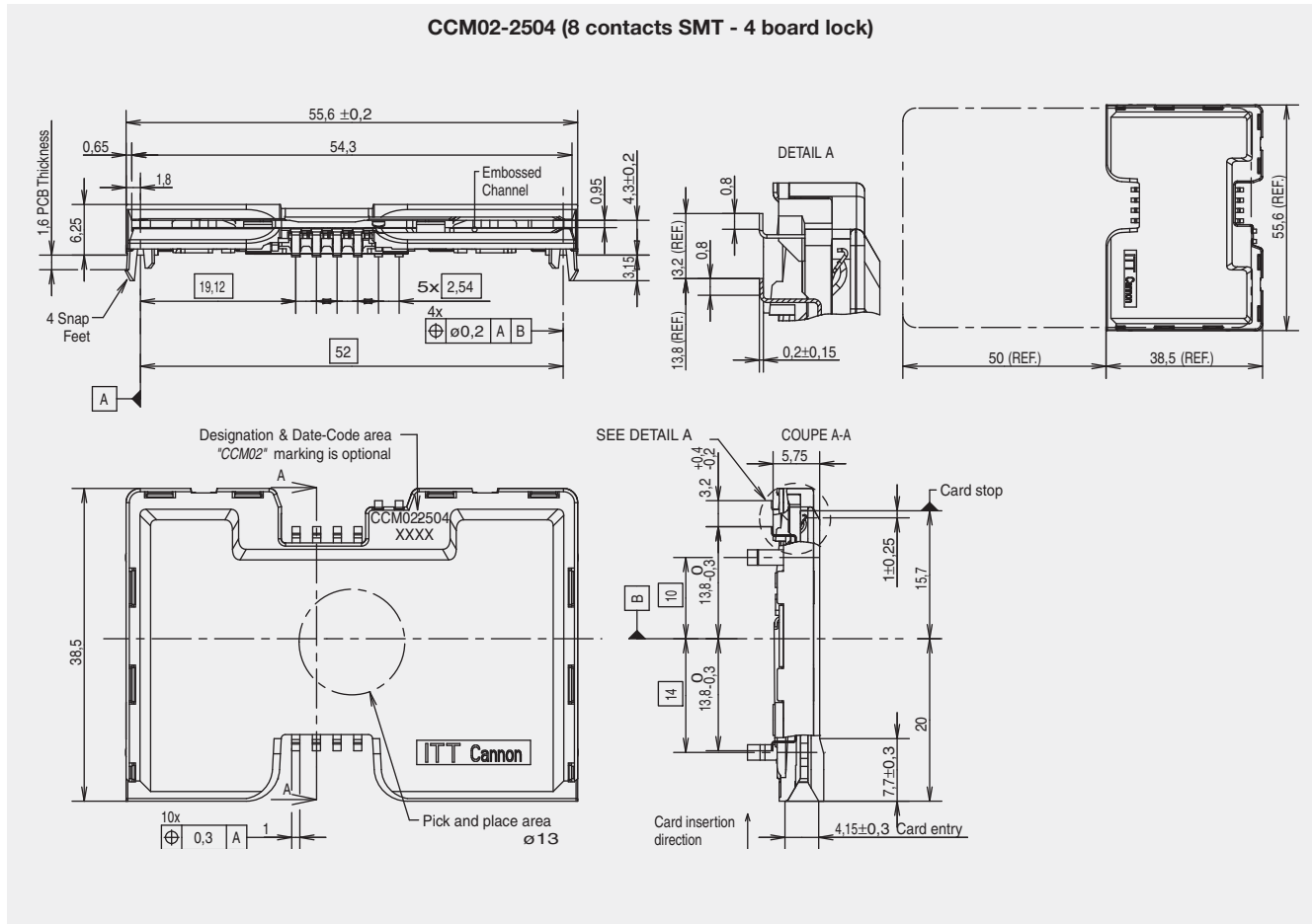
CCM02-2504 (8 contacts SMT - 4 board lock)
