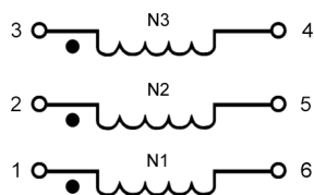
Schematic 1 (HM41-1XXXXLF)
