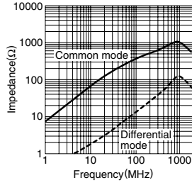
ACM3225-800-2P
