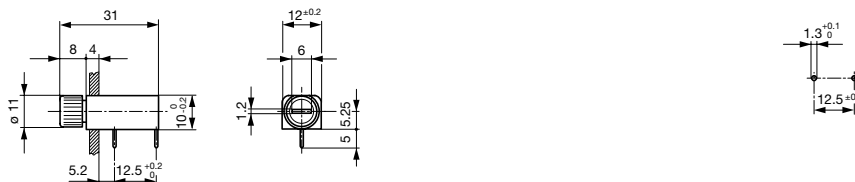
Drilling diagram
