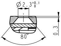
SECTION X-X SCALE 4:1
