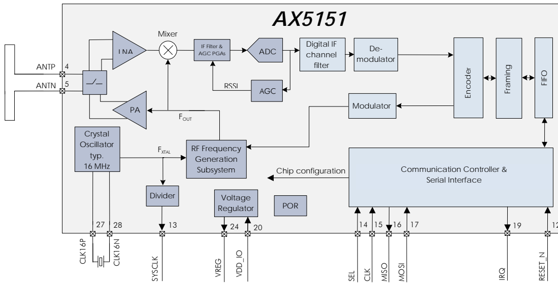
Figure 1 Functional block diagram of the AX5151
