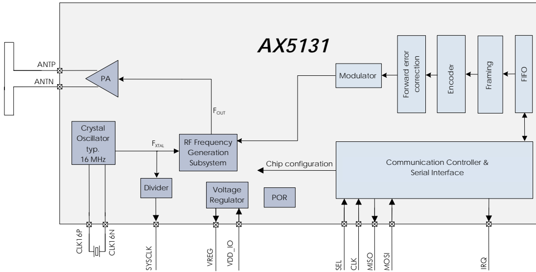
Figure 1 Functional block diagram of the AX5131
