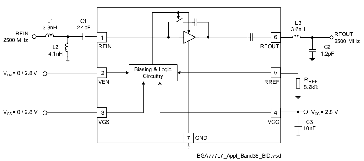
Figure 3 Application circuit with chip outline (top view)
