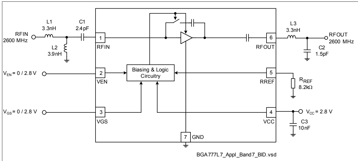
Figure 2 Application circuit with chip outline (top view)
