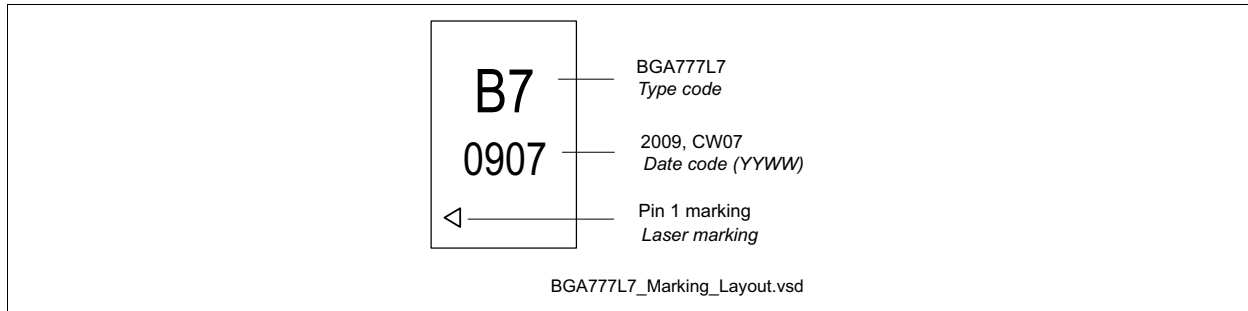
Figure 11 Marking layout
