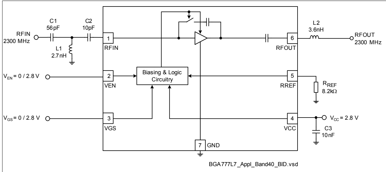
Figure 4 Application circuit with chip outline (top view)
