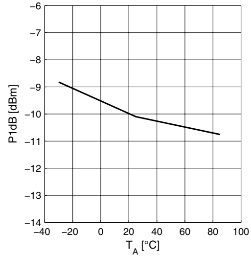
Input Compression P1dB = f(T_A)
