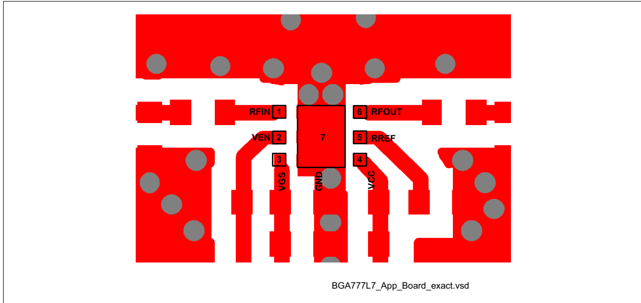
Figure 7 Detail of application board layout
