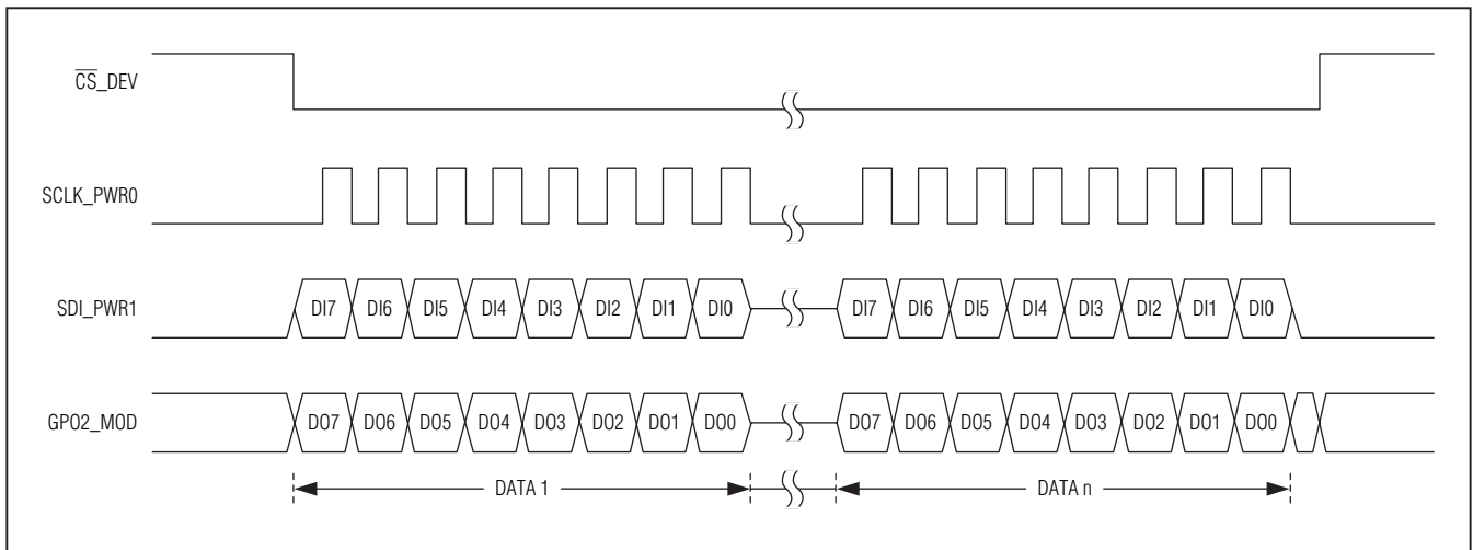
Figure 2. SPI Format
