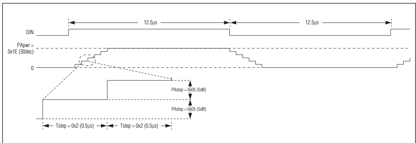
Figure 7. Digital Amplitude Shaping Timing Diagram
