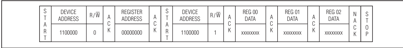
Figure 3. Example: Receive Data from Read Registers
