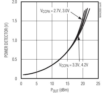
POWER DETECTOR OVER SUPPLY VOLTAGE
