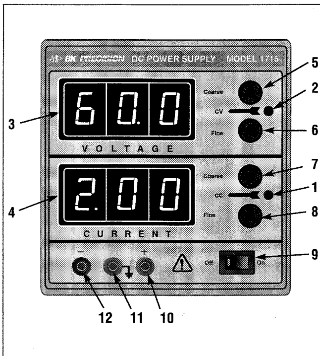
Figure 1. Front Panel Controls and Indicators.
