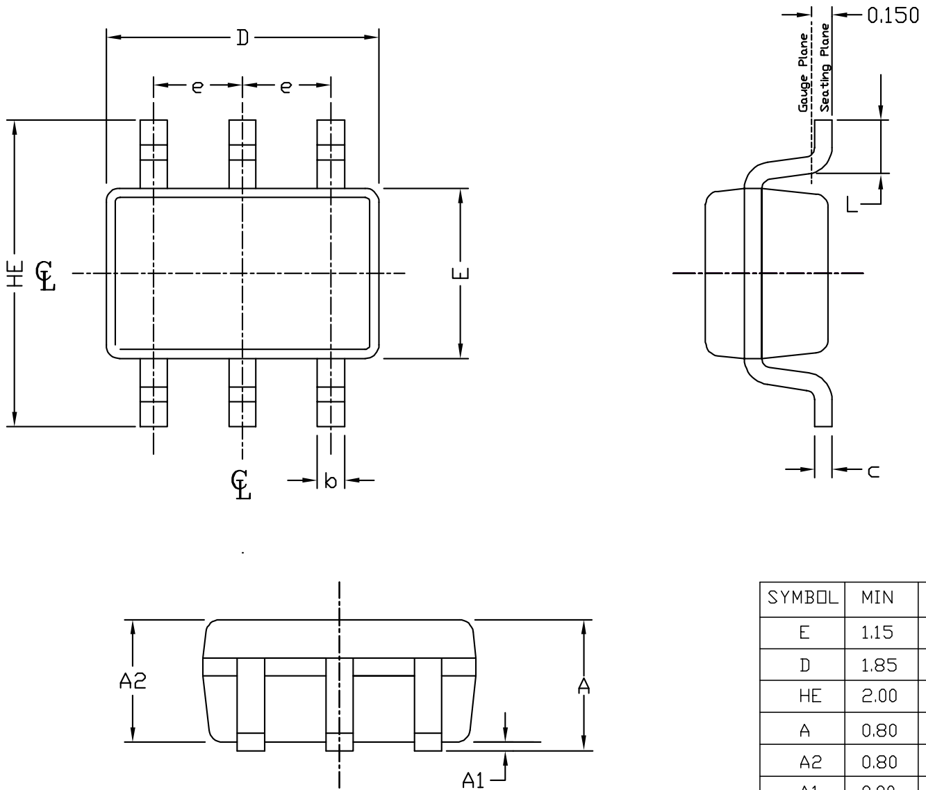
Figure 15. Package Drawing
