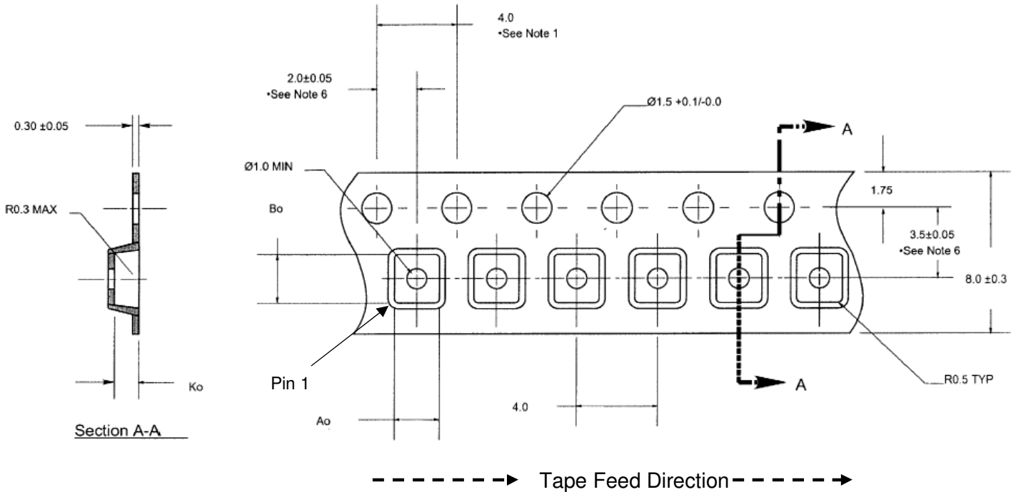
Figure 16. Tape and Reel Specifications
