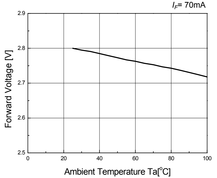
Ambient Temperature vs. Forward Voltage
