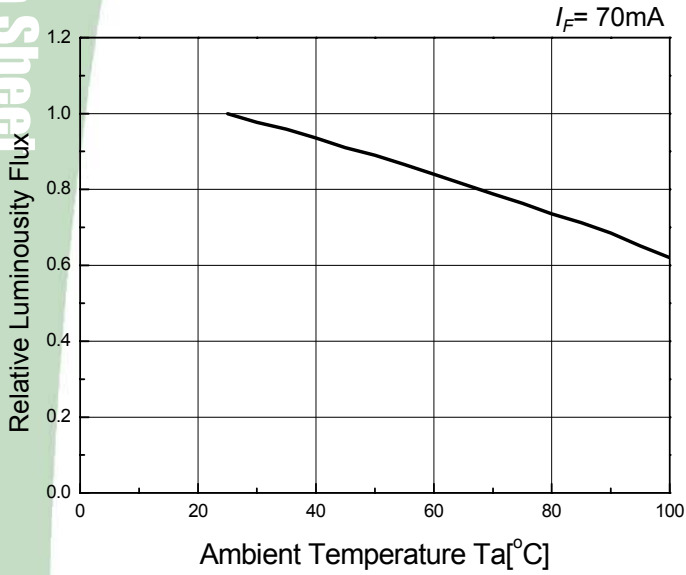
Ambient Temperature vs. Relative Flux
