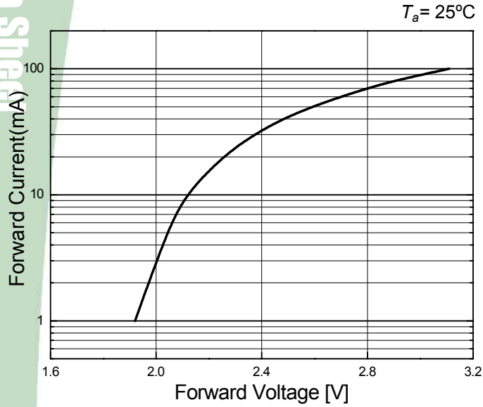
Forward Voltage vs. Forward Current
