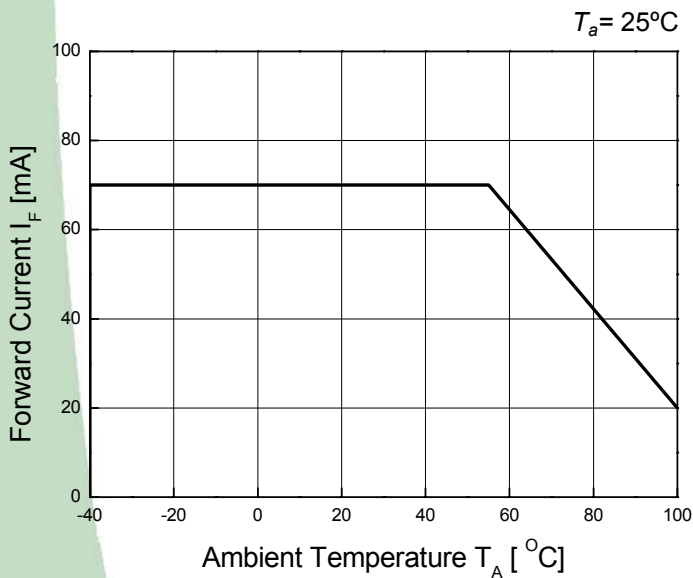
Ambient Temperature vs. Forward Current
