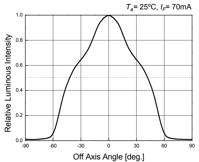
Directivity
