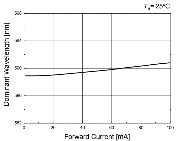
Forward Current vs. Dominant Wavelength
