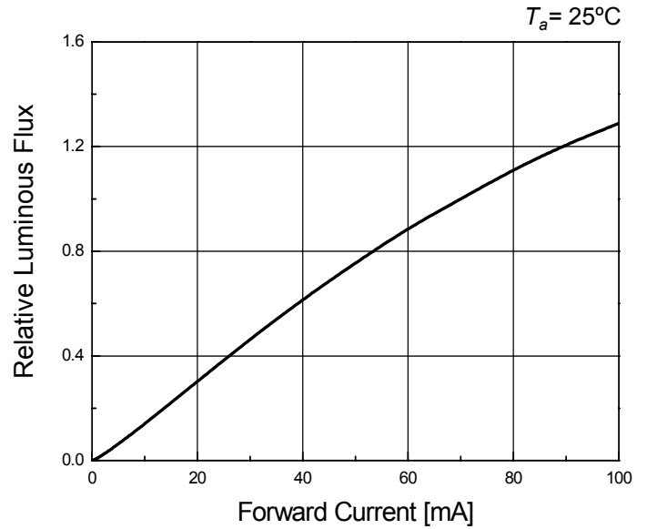
Forward Current vs. Relative Flux
