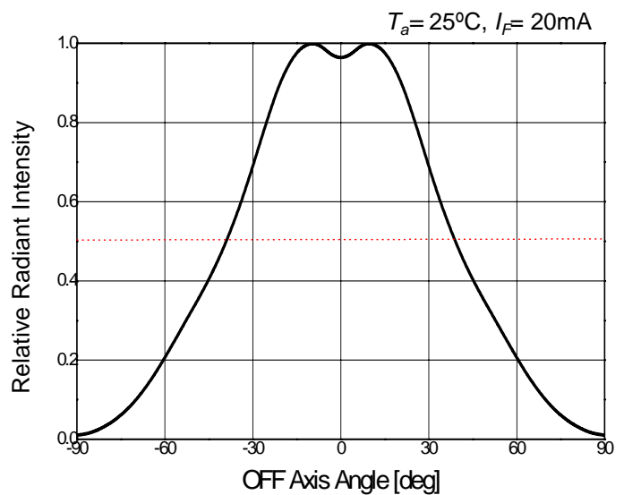
Directivity
