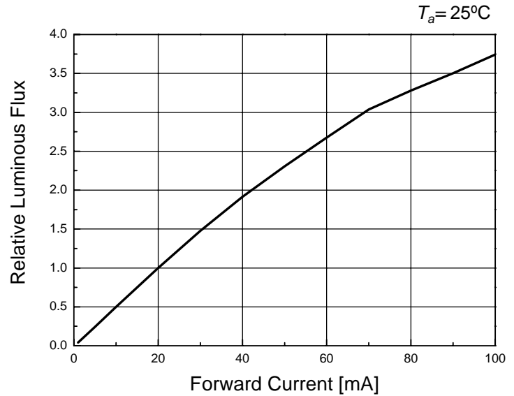
Forward Current vs. Relative Intensity
