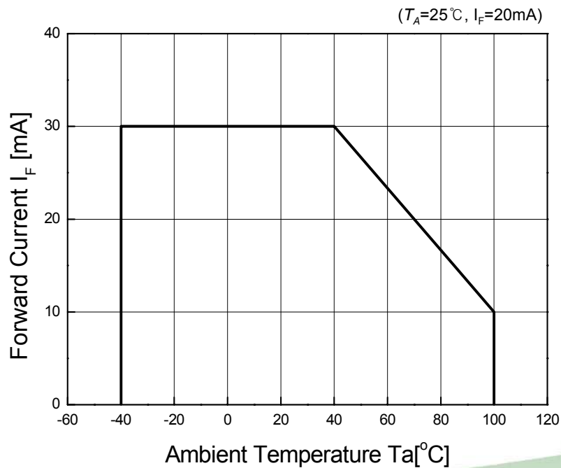
Ambient Temperature vs. Maximum Forward Current
