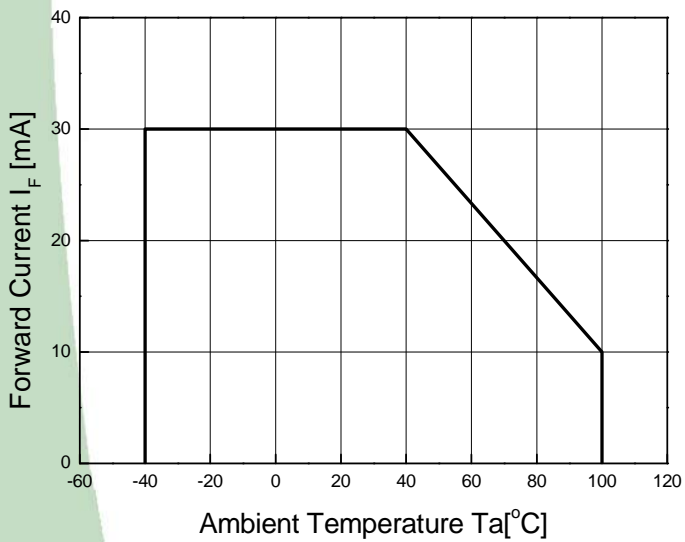
Ambient Temperature vs. Forward Current
