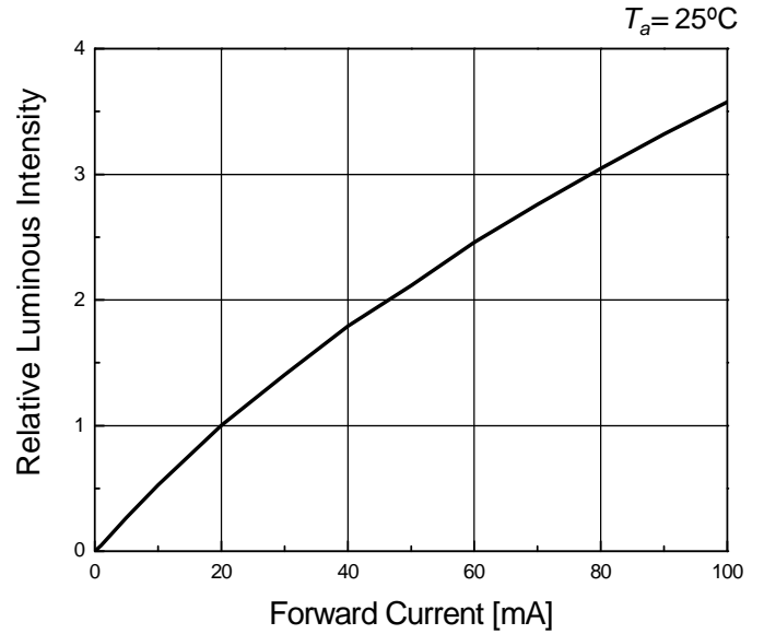
Forward Current vs. Relative Intensity
