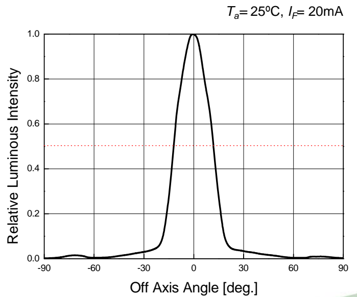
Directivity
