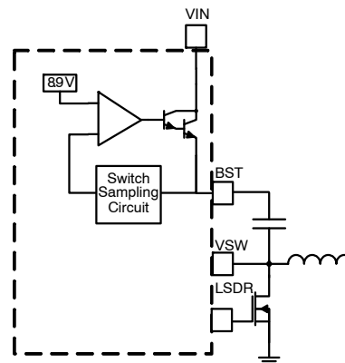
Figure 27. Boost Circuit
