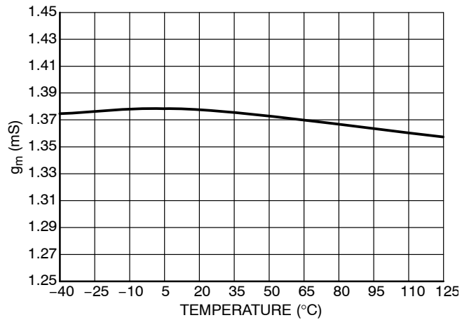
Figure 12. Transconductance vs Temperature
