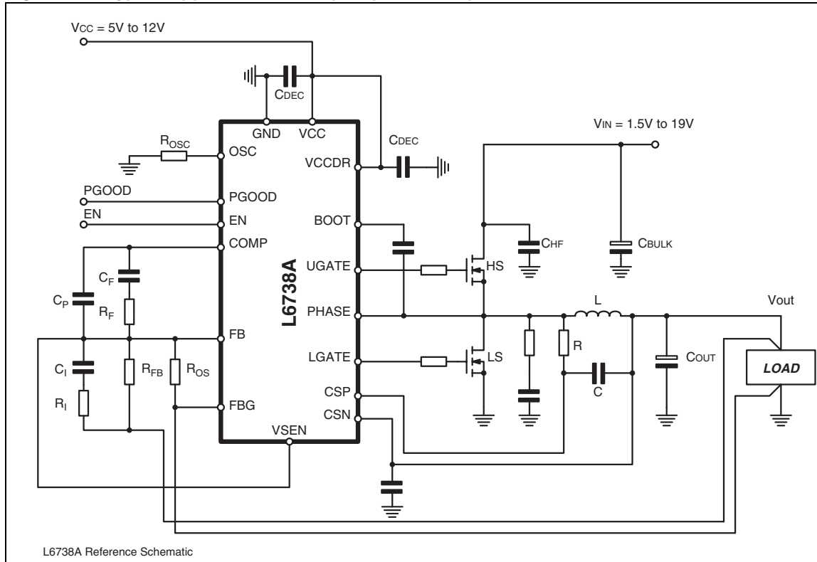
Figure 1. Typical application circuit (fast protections)
