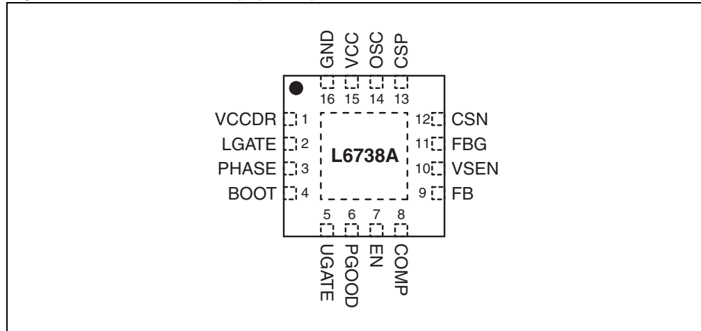
Figure 4. Pin connection (top view)
