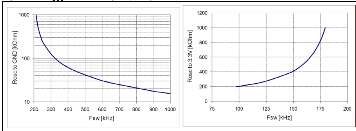
Figure 7. R_{OSC} vs. switching frequency
