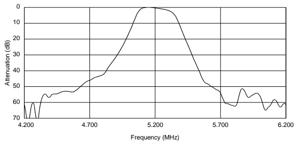
SFSKB5M20GF00-R1
