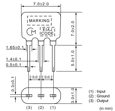
SFVLF10M7MF00-B0
