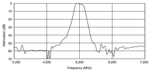
SFSKB5M20GF00-R1
