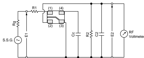
SFSKB2M30GF00-R1/SFSKB3MZ0GF00-R1
