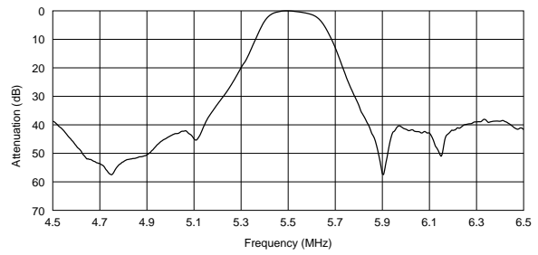
SFSKA5M50CF00-R1
