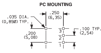
GP11MABE SPST
