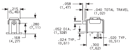
GP11MSV1BE SPST
