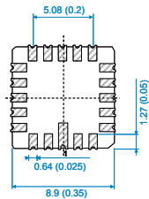
MS9000 bottom view
