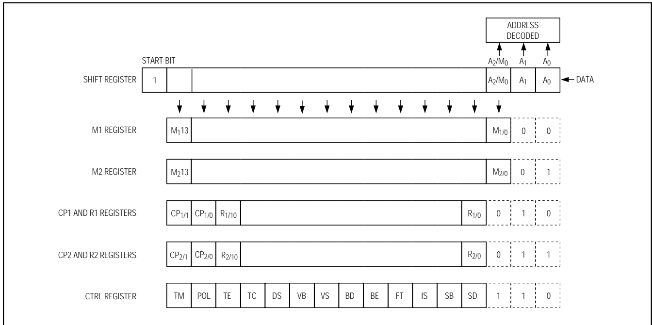
Figure 7. Programming Logic
