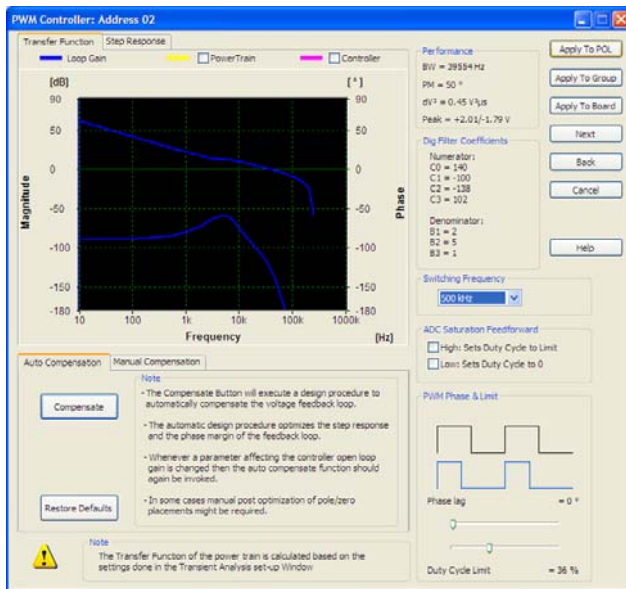
Figure 48. PWM Controller Window
