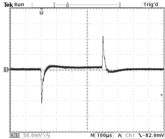
Figure 21. Vin=5V, Vout=2.5V. Bandwidth is 40kHz
