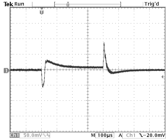
Figure 20. Vin=5V, Vout=1V. Bandwidth is 40kHz
