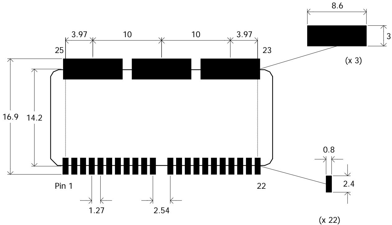
Figure 59. Recommended Pad Sizes
