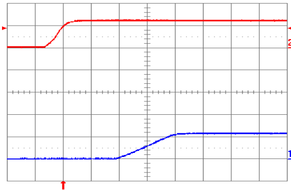
Fig. 1.2V.4: Turn-on transient for V_{out} = 1.2\text{ V} with application of V_{in} at full rated load current (resistive) and 100\ \mu\text{F} external capacitance at V_{in} = 12\text{ V} . Top trace: V_{in} (10V/div.); Bottom trace: output voltage (1 V/div.); Time scale: 2 ms/div.
