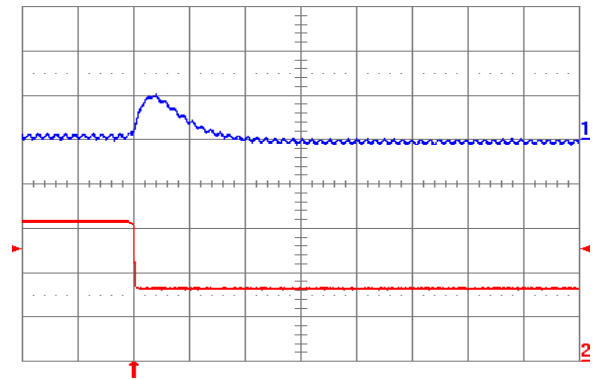
Fig. 2.5V.7: Output voltage response for V_{out} = 2.5 V to negative load current step change from 16 A to 8 A with slew rate of -5 \text{ A}/\mu\text{s} at V_{in} = 12 V. Top trace: output voltage (200 mV/div.); Bottom trace: load current (5 A/div.). C_o = 100 \mu\text{F} ceramic. Time scale: 20 \mu\text{s} /div.
