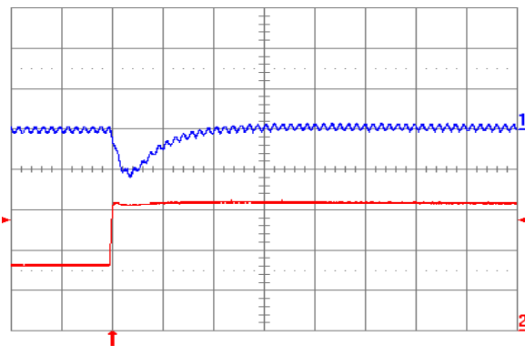
Fig. 3.3V.6: Output voltage response for V_{out} = 3.3\text{ V} to positive load current step change from 8 A to 16 A with slew rate of 5\text{ A}/\mu\text{s} at V_{in} = 12\text{ V} . Top trace: output voltage (200 mV/div.); Bottom trace: load current (5 A/div.). C_o = 100\ \mu\text{F} ceramic. Time scale: 20 \mu\text{s} /div.
