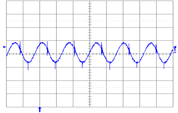
Fig. 3.3V.5: Output voltage ripple (20 mV/div.) at full rated load current into a resistive load with external capacitance 100\ \mu\text{F} ceramic and V_{in} = 12\text{ V} for V_{out} = 3.3\text{ V} . Time scale: 2 \mu\text{s} /div.
