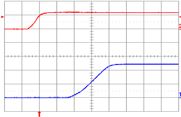
Fig. 2.5V.4: Turn-on transient for V_{out} = 2.5 V with application of V_{in} at full rated load current (resistive) and 100 \mu\text{F} external capacitance at V_{in} = 12 V. Top trace: V_{in} (10 V/div.); Bottom trace: output voltage (1 V/div.); Time scale: 2 ms/div.
