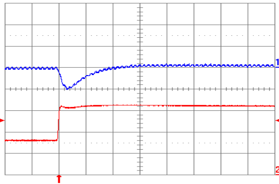
Fig. 1.8V.6: Output voltage response for V_{out} = 1.8\text{ V} to positive load current step change from 8 A to 16 A with slew rate of 5\text{ A}/\mu\text{s} at V_{in} = 12\text{ V} . Top trace: output voltage (200 mV/div.); Bottom trace: load current (5 A/div.). C_o = 100\ \mu\text{F} ceramic. Time scale: 20 \mu\text{s} /div.
