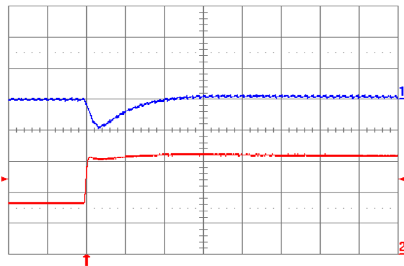
Fig. 1.5V.6: Output voltage response for V_{out} = 1.5 V to positive load current step change from 8 A to 16 A with slew rate of 5 \text{ A}/\mu\text{s} at V_{in} = 12 V. Top trace: output voltage (200 mV/div.); Bottom trace: load current (5 A/div.). C_o = 100 \mu\text{F} ceramic. Time scale: 20 \mu\text{s} /div.
