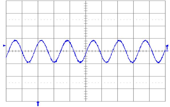
Fig. 5.0V.5: Output voltage ripple (20 mV/div.) at full rated load current into a resistive load with external capacitance 100\ \mu\text{F} ceramic and V_{in} = 12\text{ V} for V_{out} = 5.0\text{ V} . Time scale: 2 \mu\text{s} /div.
