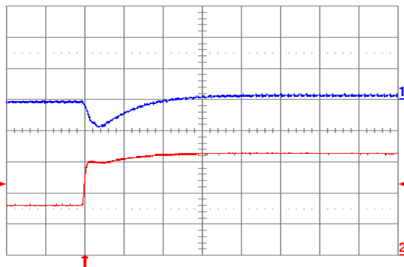
Fig. 1.0V.6: Output voltage response for V_{out} = 1.0\text{ V} to positive load current step change from 8 A to 16 A with slew rate of 5\text{ A}/\mu\text{s} at V_{in} = 12\text{ V} . Top trace: output voltage (200 mV/div.); Bottom trace: load current (5 A/div.). C_o = 100\ \mu\text{F} ceramic. Time scale: 20 \mu\text{s} /div.
