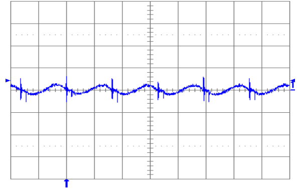
Fig. 1.2V.5: Output voltage ripple (20 mV/div.) at full rated load current into a resistive load with external capacitance 100\ \mu\text{F} ceramic and V_{in} = 12\text{ V} for V_{out} = 1.2\text{ V} . Time scale: 2 \mu\text{s} /div.
