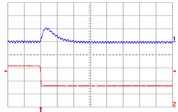
Fig. 3.3V.7: Output voltage response for V_{out} = 3.3\text{ V} to negative load current step change from 16 A to 8 A with slew rate of -5\text{ A}/\mu\text{s} at V_{in} = 12\text{ V} . Top trace: output voltage (200 mV/div.); Bottom trace: load current (5 A/div.). C_o = 100\ \mu\text{F} ceramic. Time scale: 20 \mu\text{s} /div.
