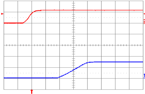
Fig. 1.5V.4: Turn-on transient for V_{out} = 1.5 V with application of V_{in} at full rated load current (resistive) and 100 \mu\text{F} external capacitance at V_{in} = 12 V. Top trace: V_{in} (10 V/div.); Bottom trace: output voltage (1 V/div.); Time scale: 2 ms/div.
