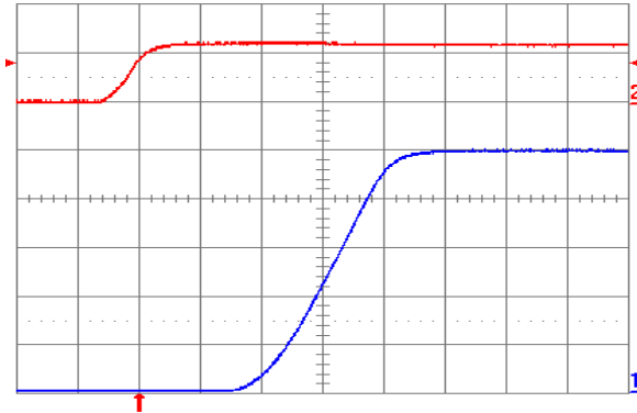
Fig. 5.0V.4: Turn-on transient for V_{out} = 5.0\text{ V} with application of V_{in} at full rated load current (resistive) and 100\ \mu\text{F} external capacitance at V_{in} = 12\text{ V} . Top trace: V_{in} (10 V/div.); Bottom trace: output voltage (1 V/div.); Time scale: 2 ms/div.
