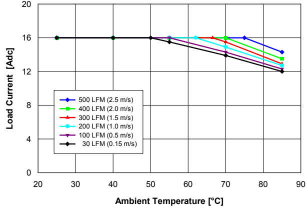
Fig. 1.5V.1: Available load current vs. ambient temperature and airflow rates for V out = 1.5 V converter mounted vertically with V in = 12 V, air flowing and maximum MOSFET temperature ≤ 120 °C.
