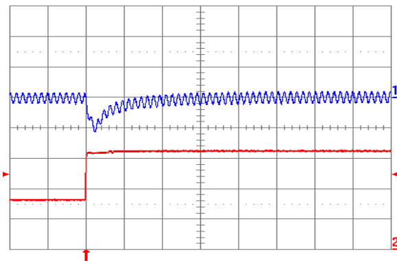
Fig. 5.0V.6: Output voltage response for V_{out} = 5.0\text{ V} to positive load current step change from 8A to 16A with slew rate of 5\text{ A}/\mu\text{s} at V_{in} = 12\text{ V} . Top trace: output voltage (200 mV/div.); Bottom trace: load current (5 A/div.). C_o = 100\ \mu\text{F} ceramic. Time scale: 20 \mu\text{s} /div.
