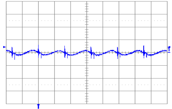
Fig. 1.0V.5: Output voltage ripple (20 mV/div.) at full rated load current into a resistive load with external capacitance 100\ \mu\text{F} ceramic and V_{in} = 12\text{ V} for V_{out} = 1.0\text{ V} . Time scale: 2 \mu\text{s} /div.
