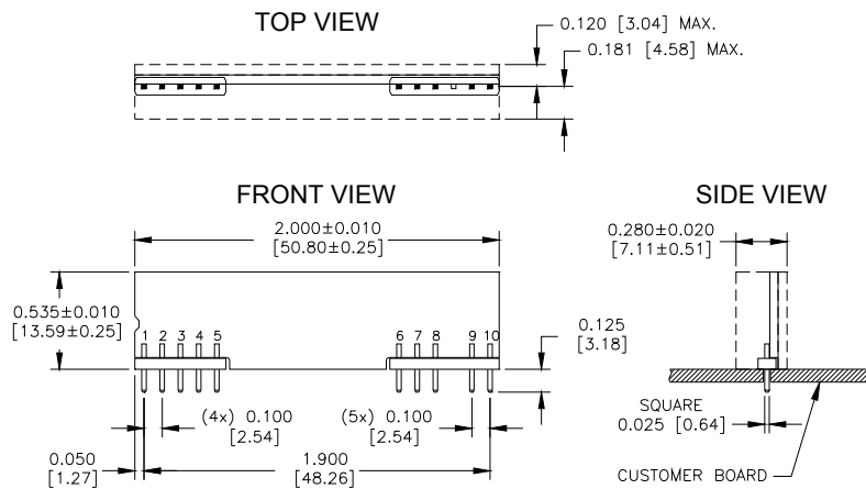
YNV12T16 Pinout (Through Hole - SIP)
