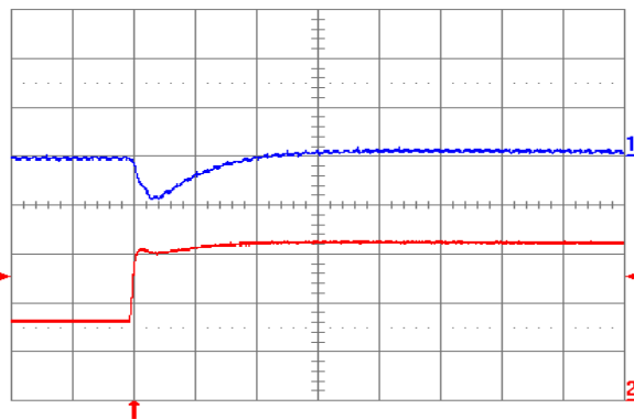
Fig. 1.2V.6: Output voltage response for V_{out} = 1.2\text{ V} to positive load current step change from 8 A to 16 A with slew rate of 5\text{ A}/\mu\text{s} at V_{in} = 12\text{ V} . Top trace: output voltage (200 mV/div.); Bottom trace: load current (5 A/div.). C_o = 100\ \mu\text{F} ceramic. Time scale: 20 \mu\text{s} /div.
