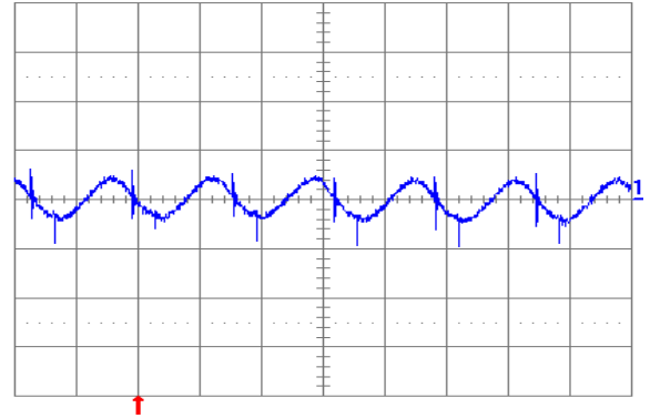
Fig. 2.5V.5: Output voltage ripple (20 mV/div.) at full rated load current into a resistive load with external capacitance 100 \mu\text{F} ceramic and V_{in} = 12 V for V_{out} = 2.5 V. Time scale: 2 \mu\text{s} /div.
