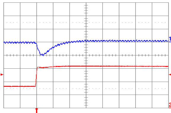
Fig. 2.5V.6: Output voltage response for V_{out} = 2.5 V to positive load current step change from 8 A to 16 A with slew rate of 5 \text{ A}/\mu\text{s} at V_{in} = 12 V. Top trace: output voltage (200 mV/div.); Bottom trace: load current (5 A/div.). C_o = 100 \mu\text{F} ceramic. Time scale: 20 \mu\text{s} /div.
