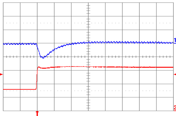
Fig. 2.0V.6: Output voltage response for V_{out} = 2.0\text{ V} to positive load current step change from 8 A to 16 A with slew rate of 5\text{ A}/\mu\text{s} at V_{in} = 12\text{ V} . Top trace: output voltage (200 mV/div.); Bottom trace: load current (5 A/div.). C_o = 100\ \mu\text{F} ceramic. Time scale: 20 \mu\text{s} /div.
