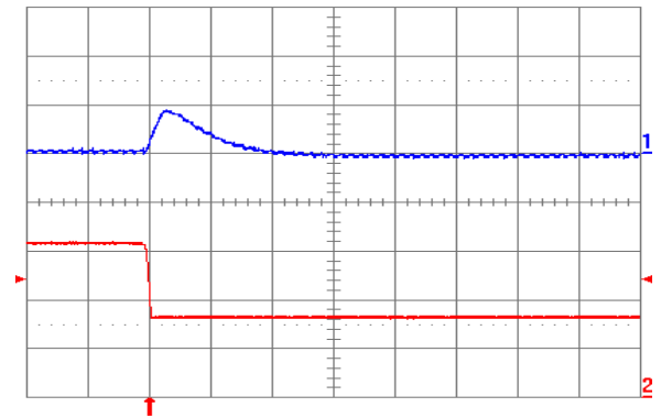
Fig. 1.5V.7: Output voltage response for V_{out} = 1.5 V to negative load current step change from 16 A to 8 A with slew rate of -5 \text{ A}/\mu\text{s} at V_{in} = 12 V. Top trace: output voltage (200 mV/div.); Bottom trace: load current (5 A/div.). C_o = 100 \mu\text{F} ceramic. Time scale: 20 \mu\text{s} /div.
