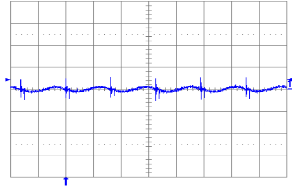
Fig. 0.7525V.5: Output voltage ripple (20 mV/div.) at full rated load current into a resistive load with external capacitance 100 \mu\text{F} ceramic and V_{in} = 12 V for V_{out} = 0.7525 V. Time scale: 2 \mu\text{s} /div.
