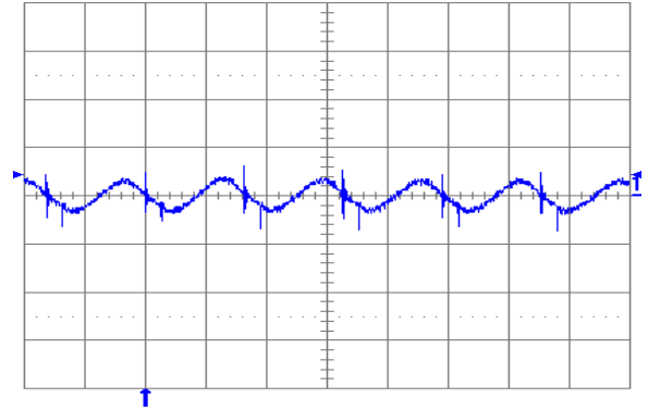
Fig. 1.8V.5: Output voltage ripple (20 mV/div.) at full rated load current into a resistive load with external capacitance 100\ \mu\text{F} ceramic and V_{in} = 12\text{ V} for V_{out} = 1.8\text{ V} . Time scale: 2 \mu\text{s} /div.
