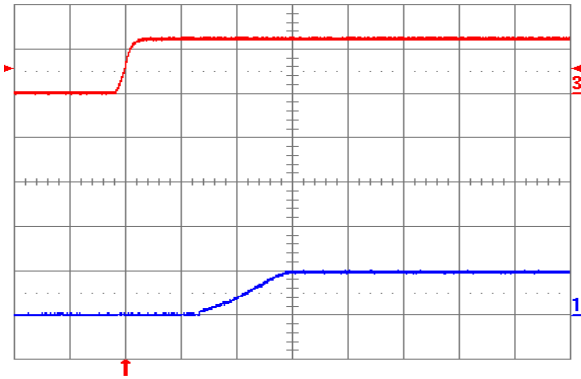
Fig. 1.0V.5: Turn-on transient for V_{out} = 1.0 V with application of V_{in} at full rated load current (resistive) and 100 \mu\text{F} external capacitance at V_{in} = 12 V. Top trace: V_{in} (10 V/div.); Bottom trace: output voltage (1 V/div.); Time scale: 5 ms/div.
