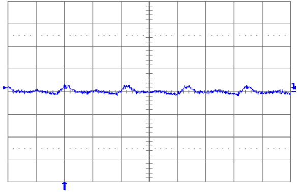
Fig. 1.2V.6: Output voltage ripple (20 mV/div.) at full rated load current into a resistive load with external capacitance 100 \mu\text{F} ceramic and V_{in} = 12 V for V_{out} = 1.2 V. Time scale: 1 \mu\text{s} /div.
