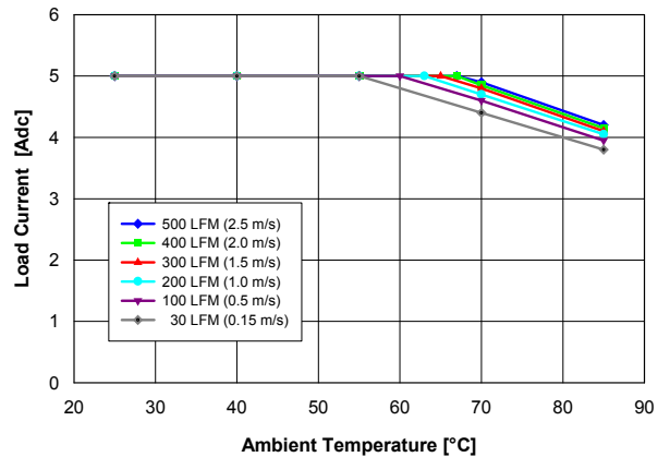
Fig. 0.7525V.2: Available load current vs. ambient temperature and airflow rates for V_{out} = 0.7525 V converter mounted horizontally with V_{in} = 12 V, and maximum MOSFET temperature \leq 120 °C.
