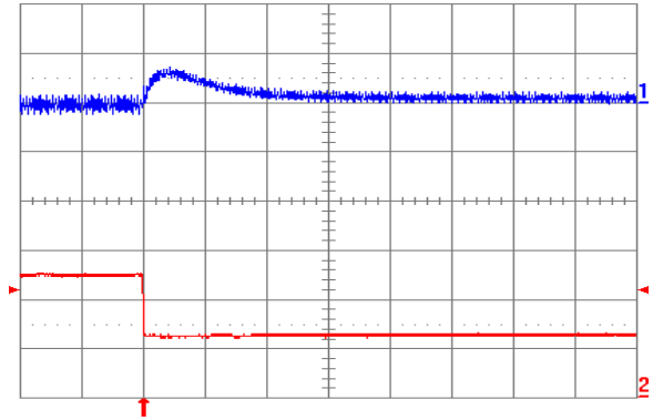
Fig. 1.5V.8: Output voltage response for V_{out} = 1.5\text{ V} to negative load current step change from 5\text{ A} to 2.5\text{ A} with slew rate of -5\text{ A}/\mu\text{s} at V_{in} = 12\text{ V} . Top trace: output voltage ( 100\text{ mV/div.} ); Bottom trace: load current ( 2\text{ A/div.} ). C_o = 100\text{ }\mu\text{F} ceramic. Time scale: 20\text{ }\mu\text{s/div.}
