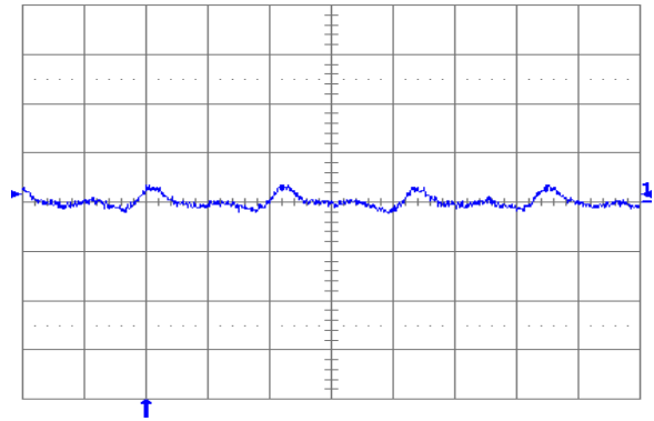
Fig. 1.8V.6: Output voltage ripple (20 mV/div.) at full rated load current into a resistive load with external capacitance 100 \mu\text{F} ceramic and V_{in} = 12 V for V_{out} = 1.8 V. Time scale: 1 \mu\text{s} /div.
