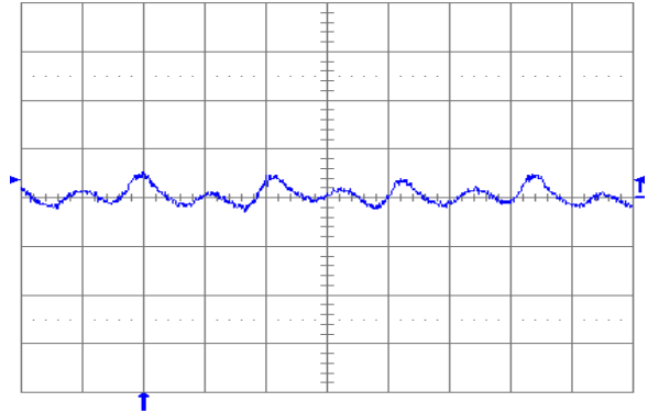
Fig. 1.5V.6: Output voltage ripple ( 20\text{ mV/div.} ) at full rated load current into a resistive load with external capacitance 100\text{ }\mu\text{F} ceramic and V_{in} = 12\text{ V} for V_{out} = 1.5\text{ V} . Time scale: 1\text{ }\mu\text{s/div.}
