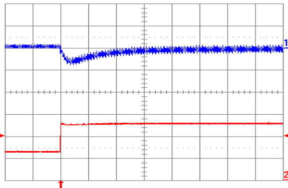
Fig. 0.7525V.7: Output voltage response for V_{out} = 0.7525\ \text{V} to positive load current step change from 2.5 A to 5 A with slew rate of 5\ \text{A}/\mu\text{s} at V_{in} = 12\ \text{V} . Top trace: output voltage (100 mV/div.); Bottom trace: load current (2 A/div.). C_o = 100\ \mu\text{F} ceramic. Time scale: 20 \mu\text{s} /div.
