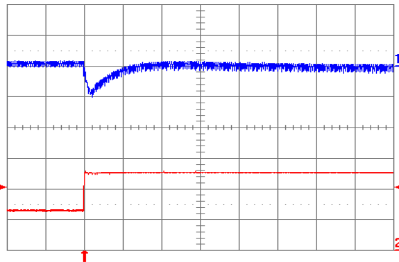
Fig. 5.0V.7: Output voltage response for V_{out} = 5.0\text{ V} to positive load current step change from 2.5 A to 5 A with slew rate of 5\text{ A}/\mu\text{s} at V_{in} = 12\text{ V} . Top trace: output voltage (100 mV/div.); Bottom trace: load current (2 A/div.). C_o = 100\text{ }\mu\text{F} ceramic. Time scale: 20 \mu\text{s} /div.
