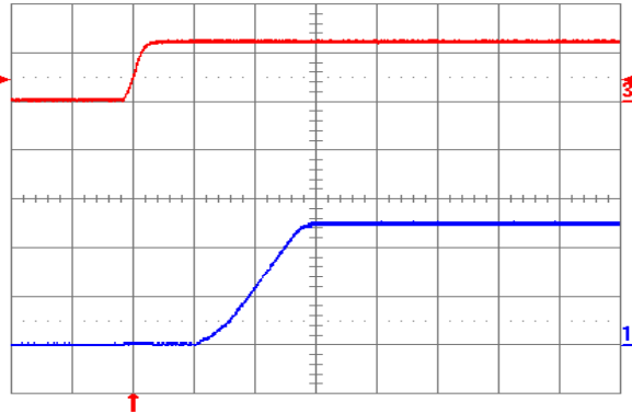
Fig. 2.5V.5: Turn-on transient for V_{out} = 2.5\text{ V} with application of V_{in} at full rated load current (resistive) and 100\ \mu\text{F} external capacitance at V_{in} = 12\text{ V} . Top trace: V_{in} (10 V/div.); Bottom trace: output voltage (1 V/div.); Time scale: 5 ms/div.
