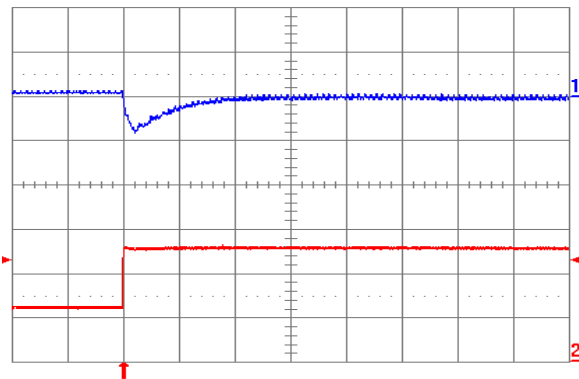
Fig. 1.8V.7: Output voltage response for V_{out} = 1.8 V to positive load current step change from 2.5 A to 5 A with slew rate of 5 \text{ A}/\mu\text{s} at V_{in} = 12 V. Top trace: output voltage (100 mV/div.); Bottom trace: load current (2 A/div.). C_o = 100 \mu\text{F} ceramic. Time scale: 20 \mu\text{s} /div.
