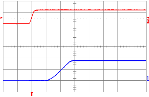
Fig. 1.8V.5: Turn-on transient for V_{out} = 1.8 V with application of V_{in} at full rated load current (resistive) and 100 \mu\text{F} external capacitance at V_{in} = 12 V. Top trace: V_{in} (10 V/div.); Bottom trace: output voltage (1 V/div.); Time scale: 5 ms/div.
