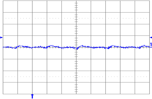
Fig. 0.7525V.6: Output voltage ripple (20 mV/div.) at full rated load current into a resistive load with external capacitance 100\ \mu\text{F} ceramic and V_{in} = 12\ \text{V} for V_{out} = 0.7525\ \text{V} . Time scale: 1 \mu\text{s} /div.
