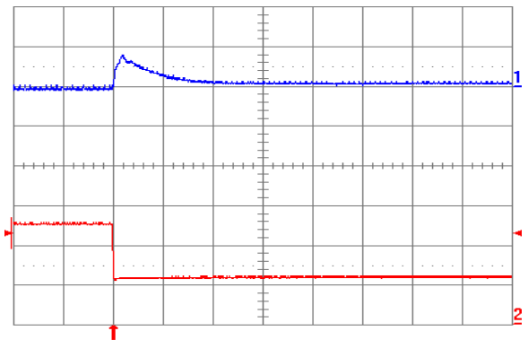
Fig. 1.8V.8: Output voltage response for V_{out} = 1.8 V to negative load current step change from 5 A to 2.5 A with slew rate of -5 \text{ A}/\mu\text{s} at V_{in} = 12 V. Top trace: output voltage (100 mV/div.); Bottom trace: load current (2 A/div.). C_o = 100 \mu\text{F} ceramic. Time scale: 20 \mu\text{s} /div.
