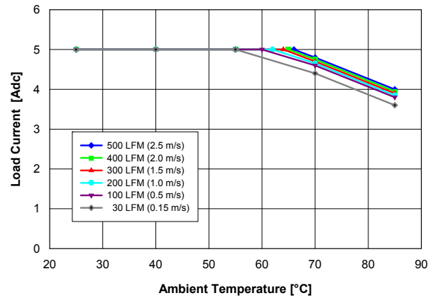
Fig. 1.0V.2: Available load current vs. ambient temperature and airflow rates for V out = 1.0 V converter mounted horizontally with V in = 12 V, and maximum MOSFET temperature ≤ 120 °C.
