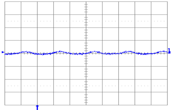
Fig. 3.3V.6: Output voltage ripple (20 mV/div.) at full rated load current into a resistive load with external capacitance 100\text{ }\mu\text{F} ceramic and V_{in} = 12\text{ V} for V_{out} = 3.3\text{ V} . Time scale: 1\text{ }\mu\text{s/div.}
