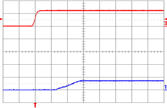
Fig. 0.7525V.5: Turn-on transient for V_{out} = 0.75250\text{V} with application of V_{in} at full rated load current (resistive) and 100\ \mu\text{F} external capacitance at V_{in} = 12\ \text{V} . Top trace: V_{in} (10 V/div.); Bottom trace: output voltage (1 V/div.); Time scale: 5 ms/div.
