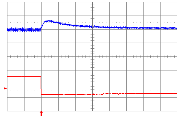
Fig. 0.7525V.8: Output voltage response for V_{out} = 0.7525\ \text{V} to negative load current step change from 5 A to 2.5 A with slew rate of -5\ \text{A}/\mu\text{s} at V_{in} = 12\ \text{V} . Top trace: output voltage (100 mV/div.); Bottom trace: load current (2 A/div.). C_o = 100\ \mu\text{F} ceramic. Time scale: 20 \mu\text{s} /div.
