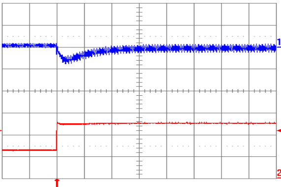
Fig. 1.5V.7: Output voltage response for V_{out} = 1.5\text{ V} to positive load current step change from 2.5\text{ A} to 5\text{ A} with slew rate of 5\text{ A}/\mu\text{s} at V_{in} = 12\text{ V} . Top trace: output voltage ( 100\text{ mV/div.} ); Bottom trace: load current ( 2\text{ A/div.} ). C_o = 100\text{ }\mu\text{F} ceramic. Time scale: 20\text{ }\mu\text{s/div.}
