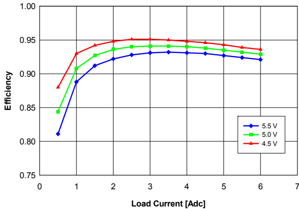
Fig. 3.3V.3: Efficiency vs. load current and input voltage for V_{out} = 3.3V converter mounted vertically or horizontally with air flowing from pin 5 to pin 1 at a rate of 200 LFM (1 m/s) and T_a = 25^{\circ}C .
