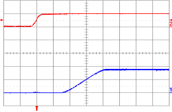
Fig. 1.8V.5: Turn-on transient for V_{out} = 1.8V with application of V_{in} at full rated load current (resistive) and 47\mu F external capacitance at V_{in} = 5V . Top trace: V_{in} (5V/div.); Bottom trace: output voltage (1V/div.); Time scale: 2ms/div.
