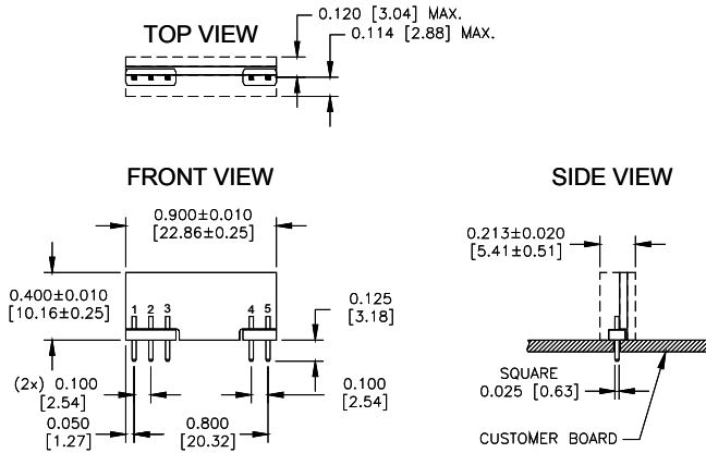
YNV05T06 Pinout (Through-Hole - SIP)
