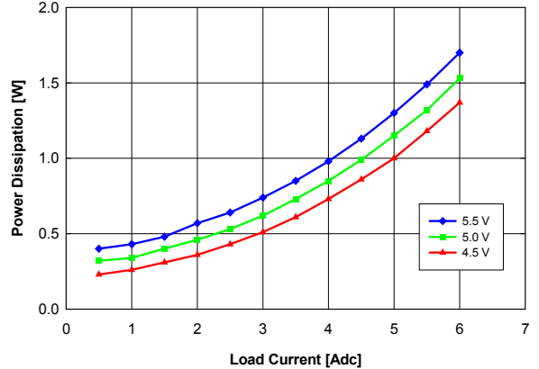
Fig. 3.3V.4: Power loss vs. load current and input voltage for V_{out} = 3.3V converter mounted vertically or horizontally with air flowing from pin 5 to pin 1 at a rate of 200 LFM (1 m/s) and T_a = 25^{\circ}C .
