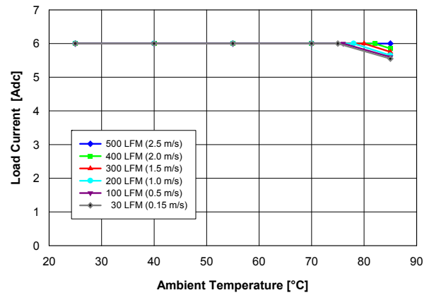
Fig. 2.5V.2: Available load current vs. ambient temperature and airflow rates for Vout = 2.5V converter mounted vertically or horizontally with Vin = 3.3V, air flowing from pin 5 to pin 1, and maximum MOSFET temperature \leq 120^{\circ}\text{C} .
