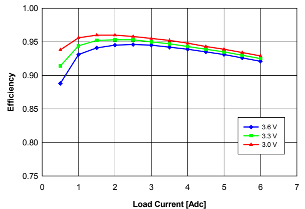
Fig. 2.5V.4: Efficiency vs. load current and input voltage for Vout = 2.5V converter mounted vertically or horizontally with air flowing from pin 5 to pin 1 at a rate of 200 LFM (1 m/s) and Ta = 25°C.
