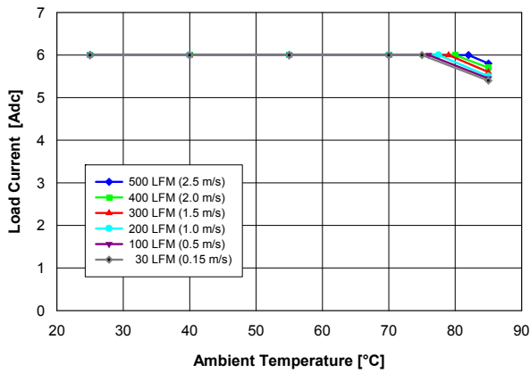
Fig. 2.5V.1: Available load current vs. ambient temperature and airflow rates for Vout = 2.5V converter mounted vertically or horizontally with Vin = 5V, air flowing from pin 5 to pin 1, and maximum MOSFET temperature \leq 120^{\circ}\text{C} .
