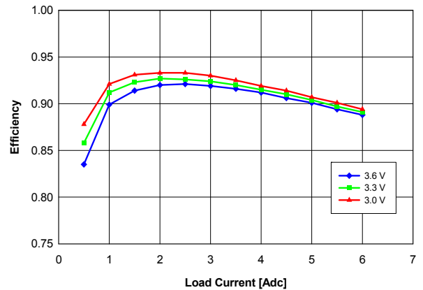
Fig. 1.8V.4: Efficiency vs. load current and input voltage for V_{out} = 1.8V converter mounted vertically or horizontally with air flowing from pin 5 to pin 1 at a rate of 200 LFM (1 m/s) and T_a = 25^{\circ}C .
