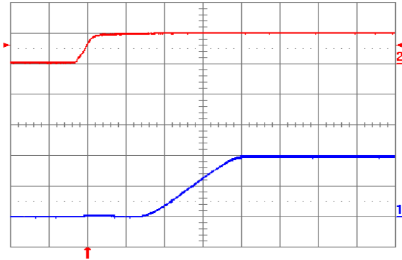
Fig. 2.0V.5: Turn-on transient for V_{out} = 2.0V with application of V_{in} at full rated load current (resistive) and 47\mu F external capacitance at V_{in} = 5V . Top trace: V_{in} (5V/div.); Bottom trace: output voltage (1V/div.); Time scale: 2ms/div.
