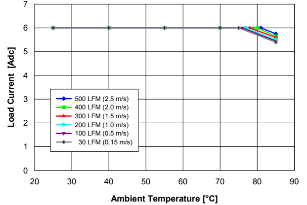
Fig. 3.3V.2: Available load current vs. ambient temperature and airflow rates for V_{out} = 3.3V converter mounted horizontally with V_{in} = 5V , air flowing from pin 1 to pin 5, and maximum MOSFET temperature \leq 120^{\circ}C .
