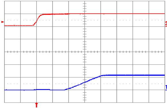
Fig. 1.2V.5: Turn-on transient for V_{out} = 1.2V with application of V_{in} at full rated load current (resistive) and 47\mu F external capacitance at V_{in} = 5V . Top trace: V_{in} (5V/div.); Bottom trace: output voltage (1V/div.); Time scale: 2ms/div.
