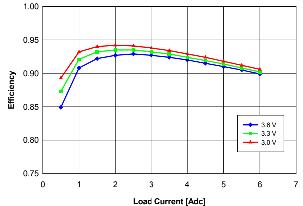
Fig. 2.0V.4: Efficiency vs. load current and input voltage for V_{out} = 2.0V converter mounted vertically or horizontally with air flowing from pin 5 to pin 1 at a rate of 200 LFM (1 m/s) and T_a = 25^{\circ}C .
