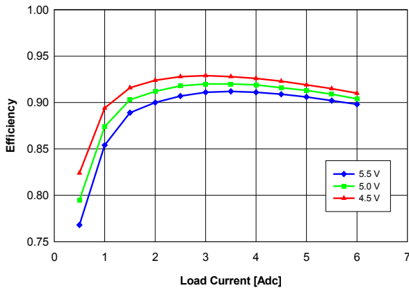
Fig. 2.5V.3: Efficiency vs. load current and input voltage for Vout = 2.5V converter mounted vertically or horizontally with air flowing from pin 5 to pin 1 at a rate of 200 LFM (1 m/s) and Ta = 25°C.
