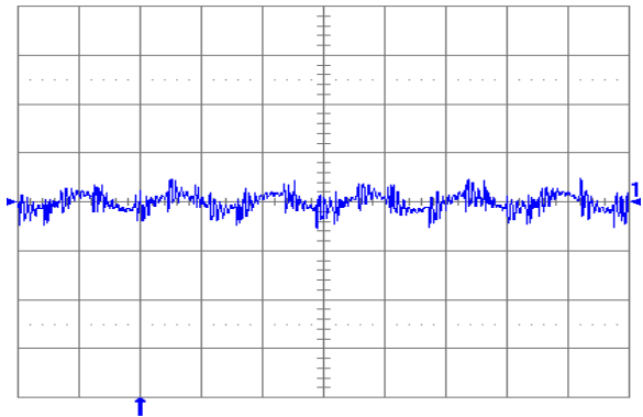
Fig. 2.0V.6: Output voltage ripple (20 mV/div.) at full rated load current into a resistive load with external capacitance 47\text{ }\mu\text{F} ceramic + 1\text{ }\mu\text{F} ceramic, and V_{in} = 5\text{ V} for V_{out} = 2.0\text{ V} . Time scale: 2 \mu\text{s} /div.
