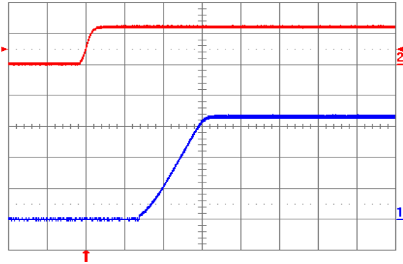
Fig. 3.3V.5: Turn-on transient for V_{out} = 3.3 V with application of V_{in} at full rated load current (resistive) and 47 \mu F external capacitance at V_{in} = 12 V. Top trace: V_{in} (10 V/div.); Bottom trace: output voltage (1 V/div.); Time scale: 5 ms/div.
