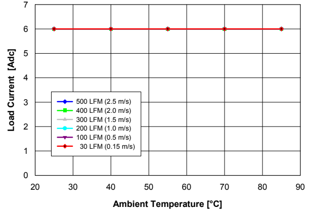
Fig. 1.0V.2: Available load current vs. ambient temperature and airflow rates for V_{out} = 1.0 V converter mounted horizontally with V_{in} = 5 V, air flowing from pin 5 to pin 1, and maximum MOSFET temperature \leq 120 °C.
