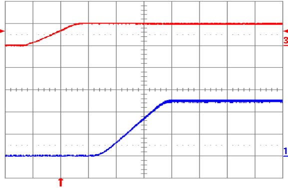
Fig. 2.5V.4: Turn-on transient for V_{out} = 2.5 V with application of V_{in} at full rated load current (resistive) and 47 \mu\text{F} external capacitance at V_{in} = 5 V. Top trace: V_{in} (5 V/div.); Bottom trace: output voltage (1V/div.); Time scale: 2 ms/div.
