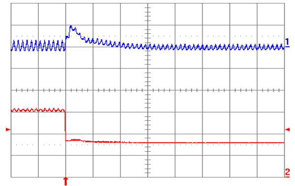
Fig. 1.0V.8: Output voltage response for V_{out} = 1.0 V to negative load current step change from 6 A to 3 A with slew rate of -5 \text{ A}/\mu\text{s} at V_{in} = 5 V. Top trace: output voltage (100 mV/div.); Bottom trace: load current (2 A/div.). C_o = 47 \mu\text{F} ceramic + 1 \mu\text{F} ceramic. Time scale: 20 \mu\text{s} /div.
