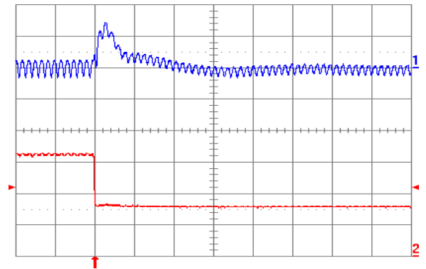
Fig. 3.3V.8: Output voltage response for V_{out} = 3.3 V to negative load current step change from 6 A to 3 A with slew rate of -5 \text{ A}/\mu\text{s} at V_{in} = 5 V. Top trace: output voltage (100 mV/div.); Bottom trace: load current (2 A/div.). C_o = 47 \mu\text{F} ceramic + 1 \mu\text{F} ceramic. Time scale: 20 \mu\text{s} /div.
