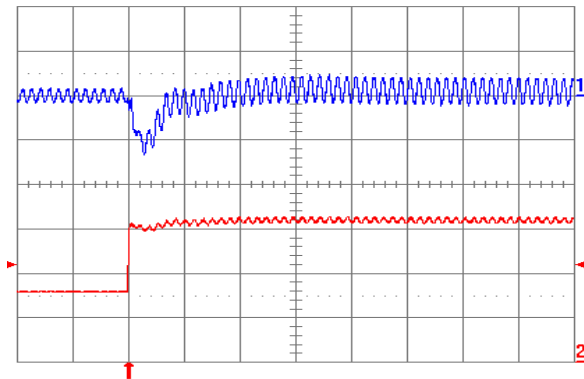
Fig. 2.0V.7: Output voltage response for V_{out} = 2.0 V to positive load current step change from 3 A to 6 A with slew rate of 5 \text{ A}/\mu\text{s} at V_{in} = 5 V. Top trace: output voltage (100 mV/div.); Bottom trace: load current (2 A/div.). C_o = 47 \mu\text{F} ceramic + 1 \mu\text{F} ceramic. Time scale: 20 \mu\text{s} /div.
