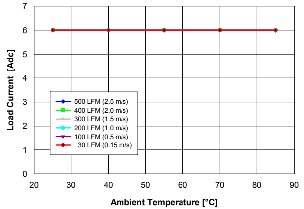
Fig. 1.8V.2: Available load current vs. ambient temperature and airflow rates for Vout = 1.8 V converter mounted horizontally with Vin = 5 V, air flowing from pin 5 to pin 1, and maximum MOSFET temperature ≤ 120 °C.
