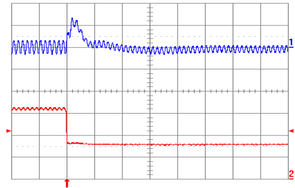
Fig. 2.5V.8: Output voltage response for V_{out} = 2.5 V to negative load current step change from 6 A to 3 A with slew rate of -5 \text{ A}/\mu\text{s} at V_{in} = 5 V. Top trace: output voltage (100 mV/div.); Bottom trace: load current (2 A/div.). C_o = 47 \mu\text{F} ceramic + 1 \mu\text{F} ceramic. Time scale: 20 \mu\text{s} /div.
