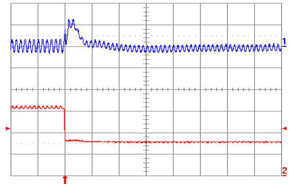
Fig. 2.0V.8: Output voltage response for V_{out} = 2.0 V to negative load current step change from 6 A to 3 A with slew rate of -5 \text{ A}/\mu\text{s} at V_{in} = 5 V. Top trace: output voltage (100 mV/div.); Bottom trace: load current (2 A/div.). C_o = 47 \mu\text{F} ceramic + 1 \mu\text{F} ceramic. Time scale: 20 \mu\text{s} /div.
