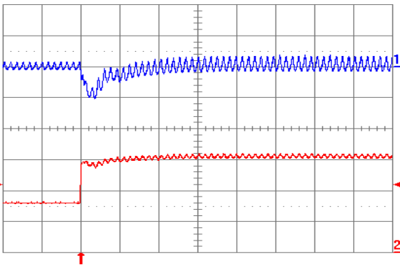
Fig. 1.0V.7: Output voltage response for V_{out} = 1.0 V to positive load current step change from 3 A to 6 A with slew rate of 5 \text{ A}/\mu\text{s} at V_{in} = 5 V. Top trace: output voltage (100 mV/div.); Bottom trace: load current (2 A/div.). C_o = 47 \mu\text{F} ceramic + 1 \mu\text{F} ceramic. Time scale: 20 \mu\text{s} /div.
