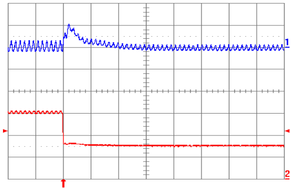
Fig. 1.2V.8: Output voltage response for V_{out} = 1.2\text{ V} to negative load current step change from 6\text{ A} to 3\text{ A} with slew rate of -5\text{ A}/\mu\text{s} at V_{in} = 5\text{ V} . Top trace: output voltage ( 100\text{ mV/div.} ); Bottom trace: load current ( 2\text{ A/div.} ). C_o = 47\text{ }\mu\text{F} ceramic + 1\text{ }\mu\text{F} ceramic. Time scale: 20\text{ }\mu\text{s/div.}
