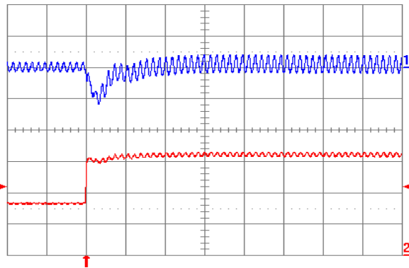
Fig. 1.5V.7: Output voltage response for V_{out} = 1.5 V to positive load current step change from 3 A to 6 A with slew rate of 5 \text{ A}/\mu\text{s} at V_{in} = 5 V. Top trace: output voltage (100 mV/div.); Bottom trace: load current (2 A/div.). C_o = 47 \mu\text{F} ceramic + 1 \mu\text{F} ceramic. Time scale: 20 \mu\text{s} /div.
