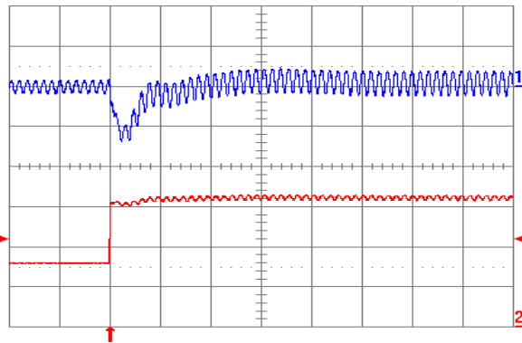
Fig. 2.5V.7: Output voltage response for V_{out} = 2.5 V to positive load current step change from 3 A to 6 A with slew rate of 5 \text{ A}/\mu\text{s} at V_{in} = 5 V. Top trace: output voltage (100 mV/div.); Bottom trace: load current (2 A/div.). C_o = 47 \mu\text{F} ceramic + 1 \mu\text{F} ceramic. Time scale: 20 \mu\text{s} /div.
