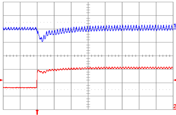
Fig. 0.7525V.7: Output voltage response for V_{out} = 0.7525 V to positive load current step change from 3 A to 6 A with slew rate of 5 \text{ A}/\mu\text{s} at V_{in} = 5 V. Top trace: output voltage (100 mV/div.); Bottom trace: load current (2 A/div.). C_o = 47 \mu\text{F} ceramic + 1 \mu\text{F} ceramic. Time scale: 20 \mu\text{s} /div.
