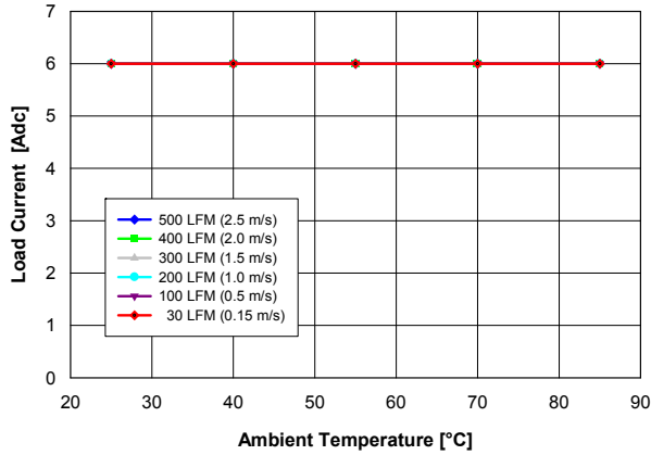
Fig. 2.5V.1: Available load current vs. ambient temperature and airflow rates for V_{out} = 2.5 V converter mounted vertically with V_{in} = 5 V, air flowing from pin 5 to pin 1, and maximum MOSFET temperature \leq 120 °C.
