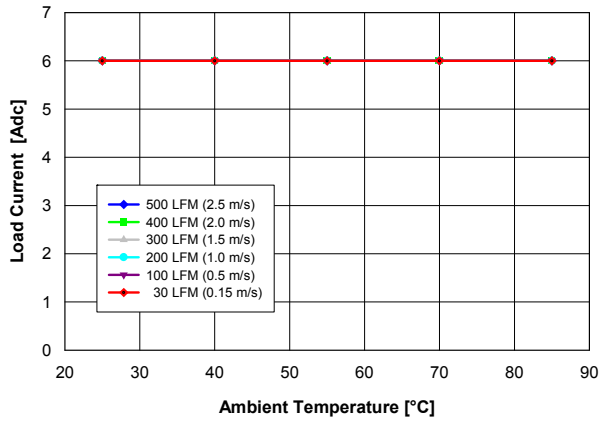
Fig. 1.8V.1: Available load current vs. ambient temperature and airflow rates for Vout = 1.8 V converter mounted vertically with Vin = 5 V, air flowing from pin 5 to pin 1, and maximum MOSFET temperature ≤ 120 °C.
