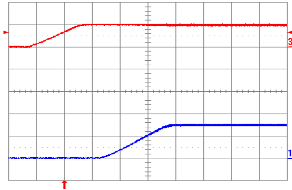
Fig. 1.5V.5: Turn-on transient for V_{out} = 1.5 V with application of V_{in} at full rated load current (resistive) and 47 \mu\text{F} external capacitance at V_{in} = 5 V. Top trace: V_{in} (5 V/div.); Bottom trace: output voltage (1 V/div.); Time scale: 2 ms/div.
