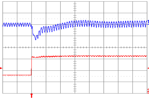
Fig. 3.3V.7: Output voltage response for V_{out} = 3.3 V to positive load current step change from 3 A to 6 A with slew rate of 5 \text{ A}/\mu\text{s} at V_{in} = 5 V. Top trace: output voltage (100 mV/div.); Bottom trace: load current (2 A/div.). C_o = 47 \mu\text{F} ceramic + 1 \mu\text{F} ceramic. Time scale: 20 \mu\text{s} /div.
