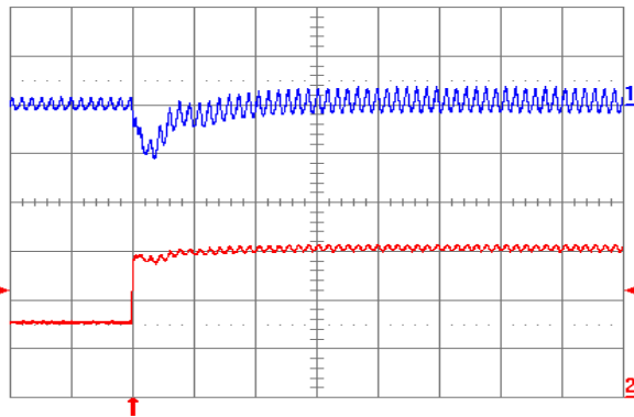
Fig. 1.2V.6: Output voltage response for V_{out} = 1.2\text{ V} to positive load current step change from 3\text{ A} to 6\text{ A} with slew rate of 5\text{ A}/\mu\text{s} at V_{in} = 5\text{ V} . Top trace: output voltage ( 100\text{ mV/div.} ); Bottom trace: load current ( 2\text{ A/div.} ). C_o = 47\text{ }\mu\text{F} ceramic + 1\text{ }\mu\text{F} ceramic. Time scale: 20\text{ }\mu\text{s/div.}
