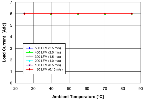
Fig. 1.0V.1: Available load current vs. ambient temperature and airflow rates for V_{out} = 1.0 V converter mounted vertically with V_{in} = 5 V, air flowing from pin 5 to pin 1, and maximum MOSFET temperature \leq 120 °C.
