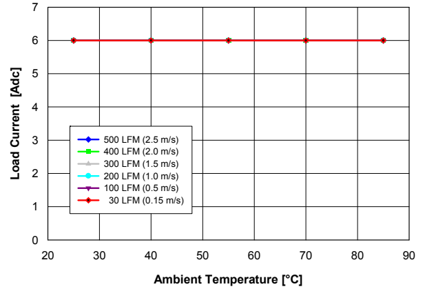
Fig. 2.5V.2: Available load current vs. ambient temperature and airflow rates for V_{out} = 2.5 V converter mounted horizontally with V_{in} = 5 V, air flowing from pin 5 to pin 1, and maximum MOSFET temperature \leq 120 °C.
