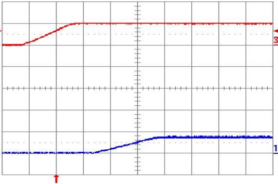
Fig. 0.7525V.4: Turn-on transient for V_{out} = 0.7525 V with application of V_{in} at full rated load current (resistive) and 47 \mu\text{F} external capacitance at V_{in} = 5 V. Top trace: V_{in} (5 V/div.); Bottom trace: output voltage (1 V/div.); Time scale: 2 ms/div.
