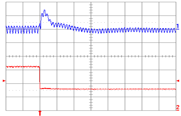
Fig. 3.3V.8: Output voltage response for V_{out} = 3.3 V to negative load current step change from 5 A to 2.5 A with slew rate of -5 \text{ A}/\mu\text{s} at V_{in} = 5 V. Top trace: output voltage (100 mV/div.); Bottom trace: load current (2 A/div.). C_o = 47 \mu\text{F} ceramic + 1 \mu\text{F} ceramic. Time scale: 20 \mu\text{s} /div.
