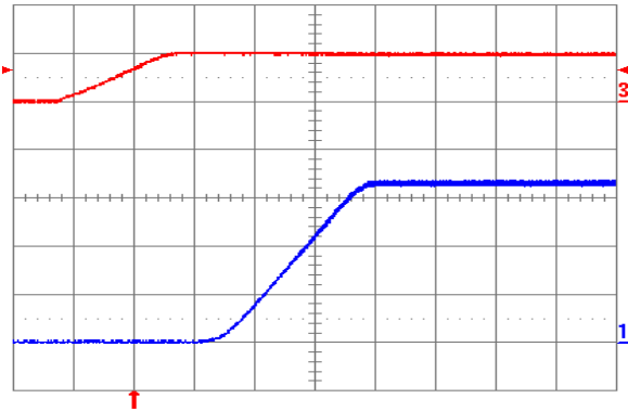
Fig. 3.3V.5: Turn-on transient for V_{out} = 3.3 V with application of V_{in} at full rated load current (resistive) and 47 \mu\text{F} external capacitance at V_{in} = 5 V. Top trace: V_{in} (5 V/div.); Bottom trace: output voltage (1 V/div.); Time scale: 2 ms/div.
