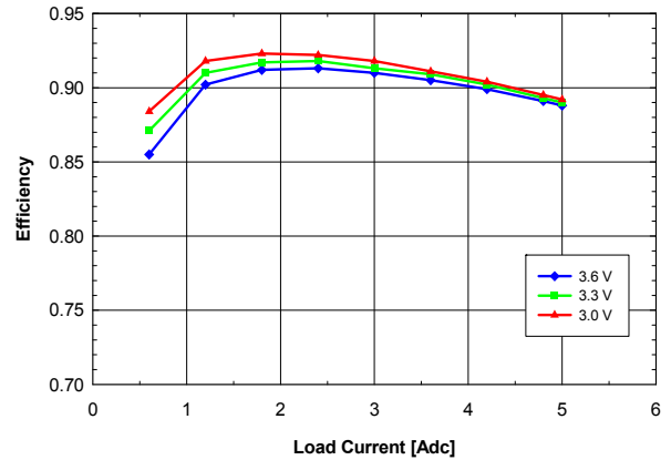
Fig. 1.5V.4: Efficiency vs. load current and input voltage for V_{out} = 1.5\text{ V} converter mounted vertically with air flowing from pin 5 to pin 1 at a rate of 200 LFM (1 m/s) and T_a = 25\text{ }^{\circ}\text{C} .
