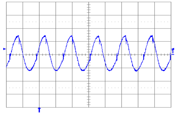
Fig. 1.5V.6: Output voltage ripple (20 mV/div.) at full rated load current into a resistive load with external capacitance 10\ \mu\text{F} ceramic + 1\ \mu\text{F} ceramic and V_{in} = 5\text{ V} for V_{out} = 1.5\text{ V} . Time scale: 2 \mu\text{s} /div.
