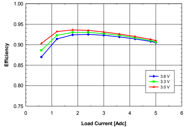
Fig. 1.8V.4: Efficiency vs. load current and input voltage for V_{out} = 1.8\text{ V} converter mounted vertically with air flowing from pin 5 to pin 1 at a rate of 200 LFM (1 m/s) and T_a = 25\text{ }^{\circ}\text{C} .
