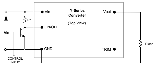
Fig. C: Circuit configuration for ON/OFF function.
