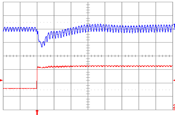
Fig. 3.3V.7: Output voltage response for V_{out} = 3.3 V to positive load current step change from 2.5 A to 5 A with slew rate of 5 \text{ A}/\mu\text{s} at V_{in} = 5 V. Top trace: output voltage (100 mV/div.); Bottom trace: load current (2 A/div.). C_o = 47 \mu\text{F} ceramic + 1 \mu\text{F} ceramic. Time scale: 20 \mu\text{s} /div.
