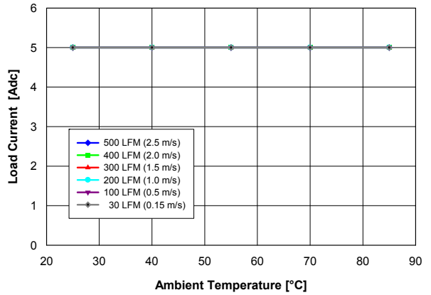
Fig. 0.7525V.2: Available load current vs. ambient temperature and airflow rates for V_{out} = 0.7525 V converter mounted horizontally with V_{in} = 5 V, air flowing from pin 5 to pin 1, and maximum MOSFET temperature \leq 120 °C.
