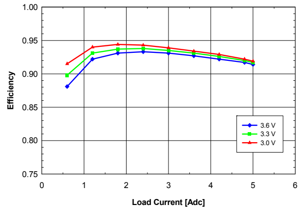
Fig. 2.0V.4: Efficiency vs. load current and input voltage for V_{out} = 2.0 V converter mounted vertically with air flowing from pin 5 to pin 1 at a rate of 200 LFM (1 m/s) and T_a = 25 °C.
