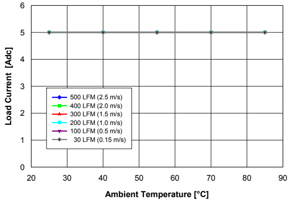
Fig. 0.7525V.1: Available load current vs. ambient temperature and airflow rates for V_{out} = 0.7525 V converter mounted vertically with V_{in} = 5 V, air flowing from pin 5 to pin 1, and maximum MOSFET temperature \leq 120 °C.
