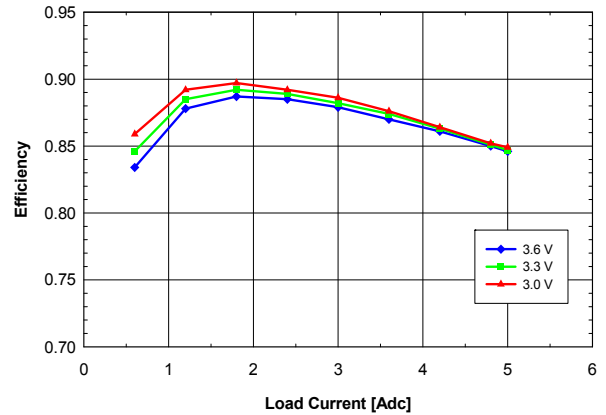
Fig. 1.0V.4: Efficiency vs. load current and input voltage for V_{out} = 1.0\text{ V} converter mounted vertically with air flowing from pin 5 to pin 1 at a rate of 200 LFM (1m/s) and T_a = 25\text{ }^{\circ}\text{C} .
