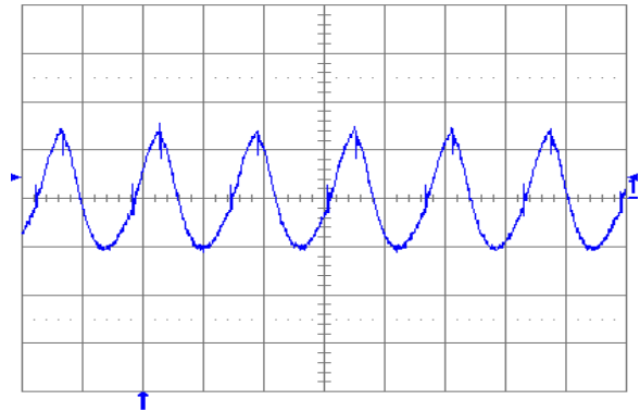
Fig. 1.2V.6: Output voltage ripple ( 20\text{ mV/div.} ) at full rated load current into a resistive load with external capacitance 10\text{ }\mu\text{F} ceramic + 1\text{ }\mu\text{F} ceramic and V_{in} = 5\text{ V} for V_{out} = 1.2\text{ V} . Time scale: 2\text{ }\mu\text{s/div.}
