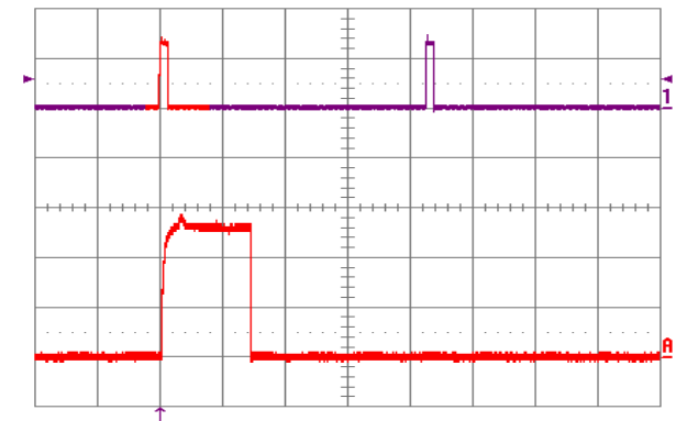
Figure 15. Load current (top trace, 20 \text{ A}/\text{div} ., 50 \text{ ms}/\text{div} .) into a 10 \text{ m}\Omega short circuit during restart, at V_{in} = 48 \text{ V} . Bottom trace ( 10 \text{ A}/\text{div} ., 5 \text{ ms}/\text{div} .) is an expansion of the on-time portion of the top trace
