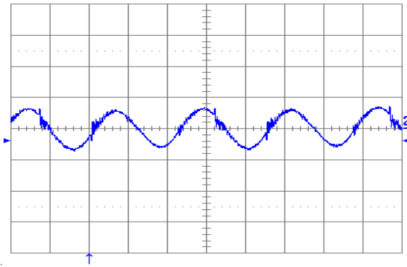
Figure 10. Output voltage ripple (50 mV/div.) at full rated load current into a resistive load with C_o = 10 \mu\text{F} tantalum + 1 \mu\text{F} ceramic and V_{in} = 48 \text{ V} . Time scale: 1 \mu\text{s}/\text{div} .
