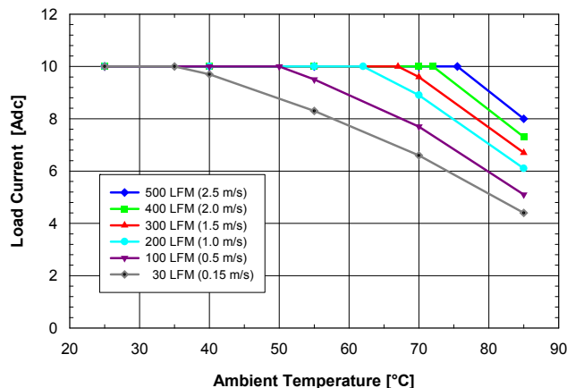
Fig. 5.0V.1: Available load current vs. ambient air temperature and airflow rates for SQ48T10050 converter with D height pins mounted vertically with V_{in} = 48\text{ V} , air flowing from pin 3 to pin 1, and maximum FET temperature \leq 120^\circ\text{C} .
