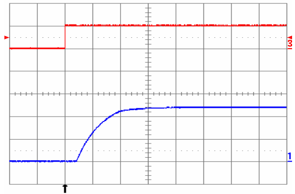
Fig. 8: Turn-on transient at full rated load current (resistive) plus 2,200 µF at V_{in} = 48\text{ V} , triggered via ON/OFF pin. Top trace: ON/OFF signal (5 V/div.). Bottom trace: output voltage (5 V/div.). Time scale: 2 ms/div.
