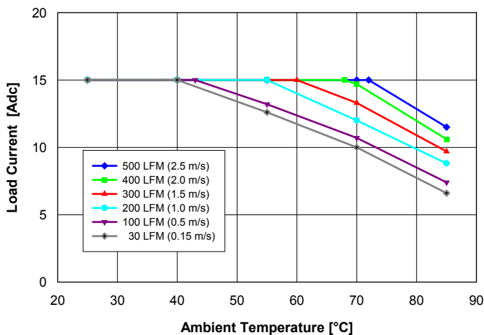
Fig. 11: Available load current vs. ambient air temperature and airflow rates for converter mounted vertically with V_{in} = 27\text{ V} , air flowing from pin 3 to pin 1 and maximum FET temperature \leq 105^{\circ}\text{C} .
