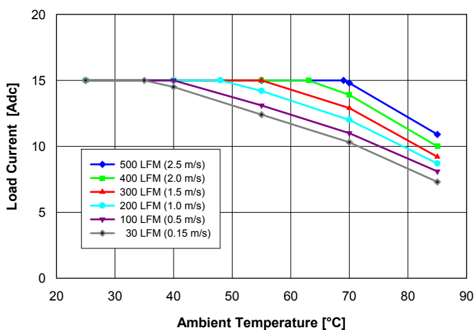
Fig. 13: Available load current vs. ambient temperature and airflow rates for converter mounted horizontally with V_{in} = 27\text{ V} , air flowing from pin 3 to pin 4 and maximum FET temperature \leq 105^{\circ}\text{C} .
