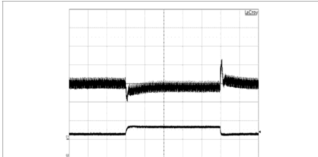
Output voltage response to load current step- change (7.5-22.5-7.5 A) at: T_{ref} = +25^\circ\text{C} , V_i = 53\text{ V} . Top trace: output voltage (100 mV/div.). Bottom trace: load current (30 A/div.). Time scale: (0.1 ms/div.).
